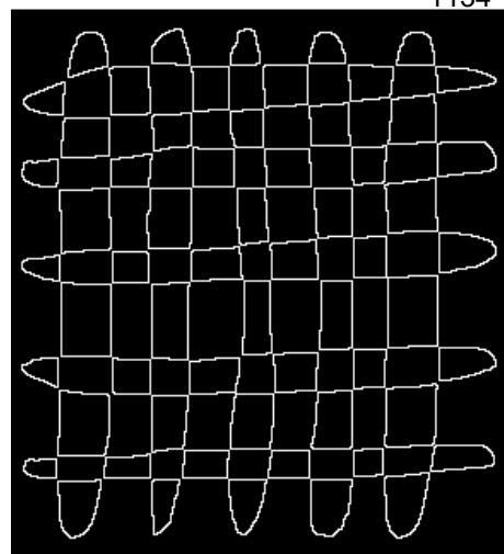
Fig. 38 Y-partition, 60 contours
