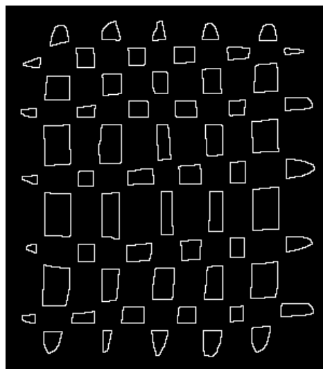
Fig. 48 Y-partition, 60 contours
