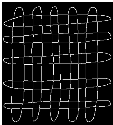
Fig. 37 X-partition, 42 contours
