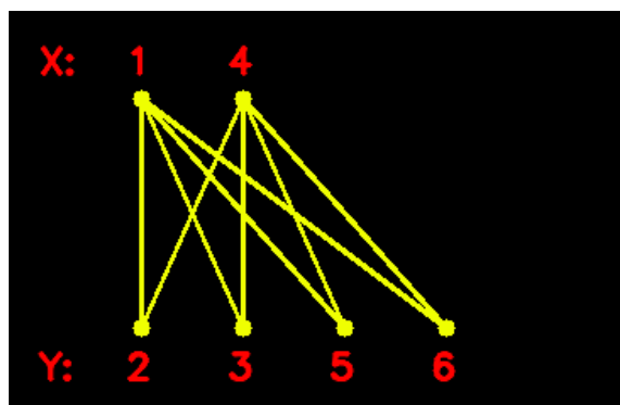
Fig. 6 bi-partitioned graph
