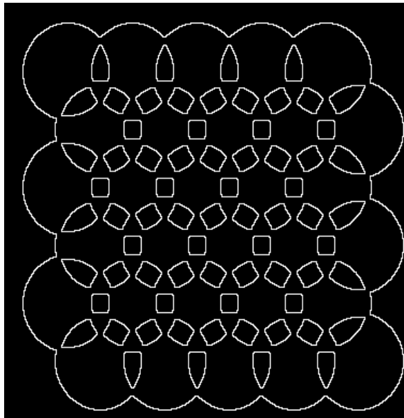
Fig. 32 X-partition, 70 contours
