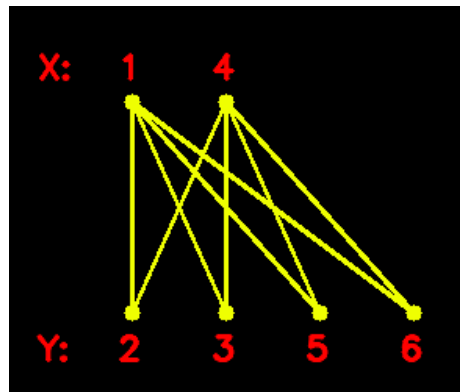
Fig. 13 Bi-partitioned graph
