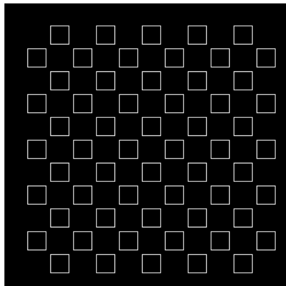
Fig. 23 Y-partition, 60 contours
