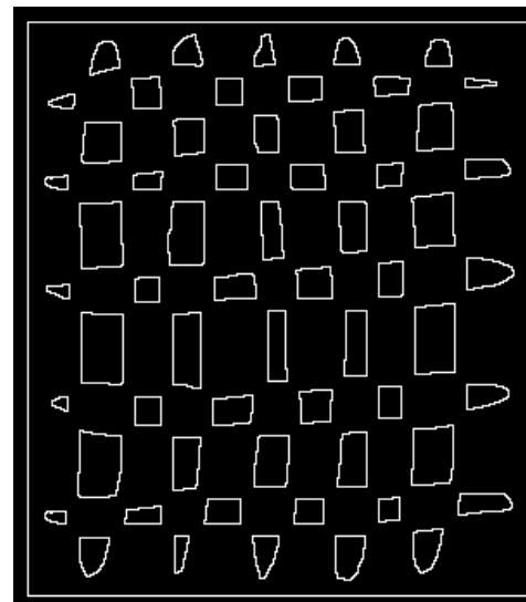
Fig. 52 X-partition, 61 contours
