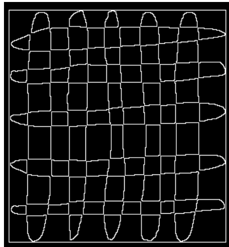
Fig. 42 X-partition, 61 contours
