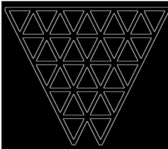
Fig. 56 35 contours extracted
