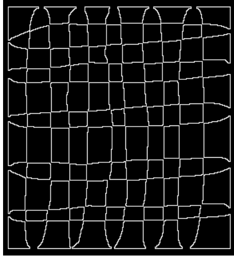
Fig. 43 Y-partition, 61 contours
