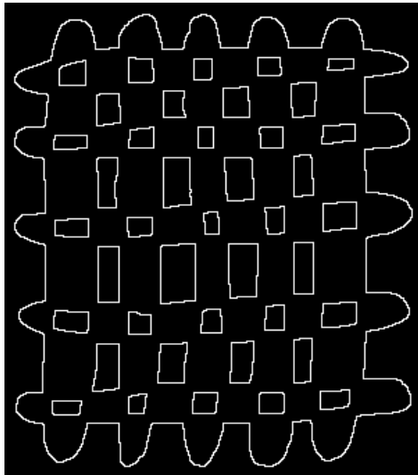
Fig. 47 X-partition, 42 contours
