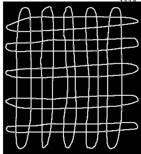
Fig. 36 102 contours extracted
