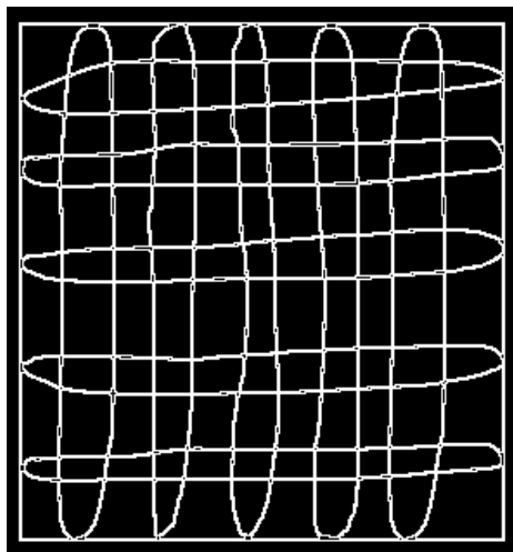
Fig. 41 122 contours extracted
