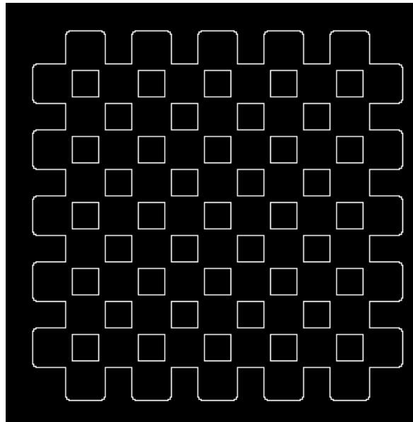
Fig. 22 X-partition, 42 contours
