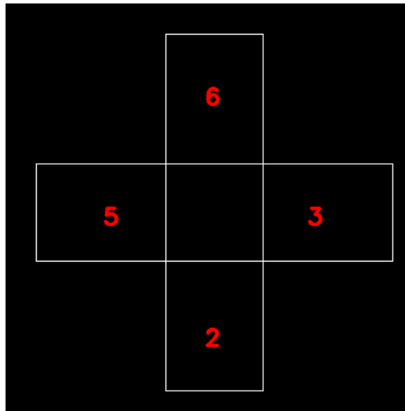
Fig. 5 Y-partition, 4 contours
