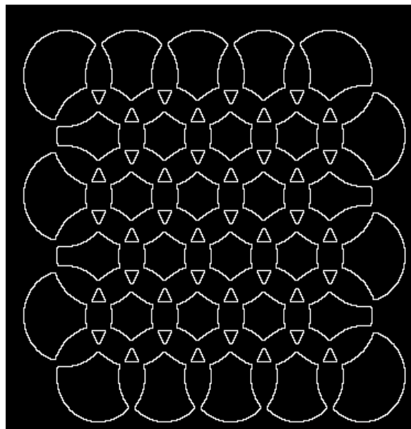
Fig. 33 Y-partition, 70 contours
