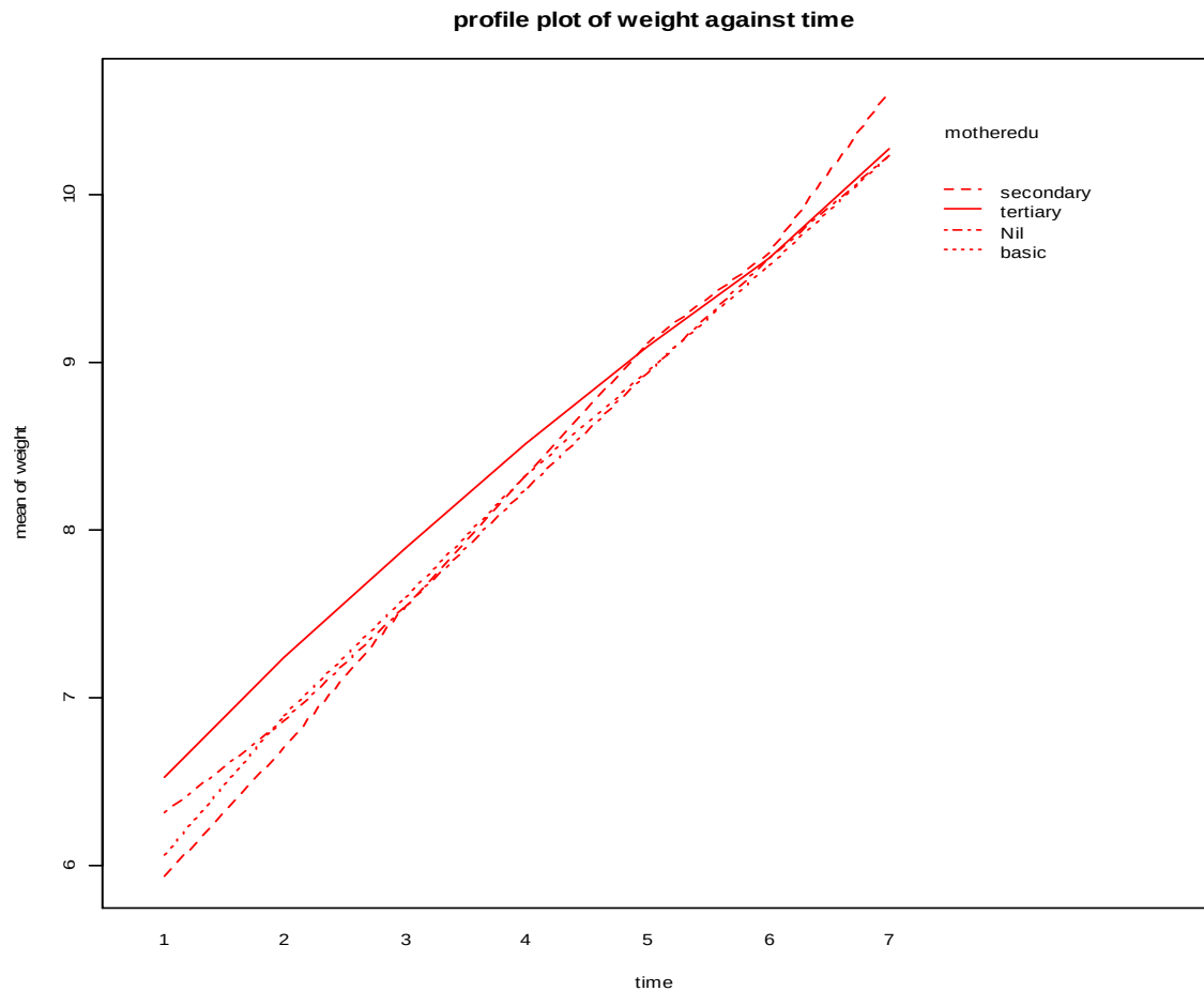
figure 4.4 Profile plot of mean weight babies by mother's educational level
