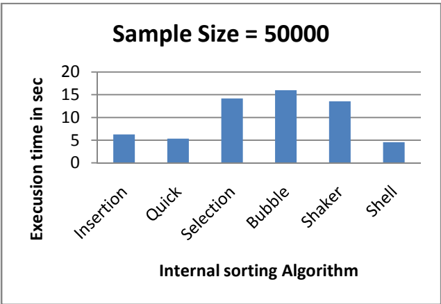
Figure 2: Execution time performance between ISAs over 50,000 data samples
