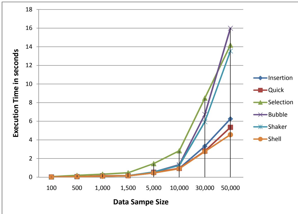
Figure 4: General overview of growth rate based on data size and execution time in sec of ISAs
