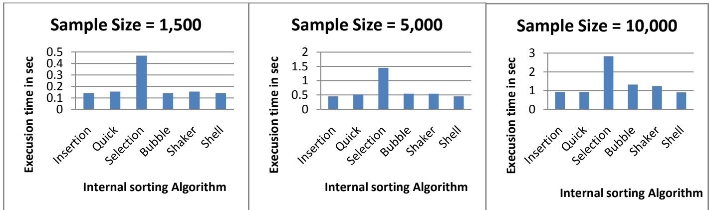
Figure 3: Comparison of ISA across data sample sizes
