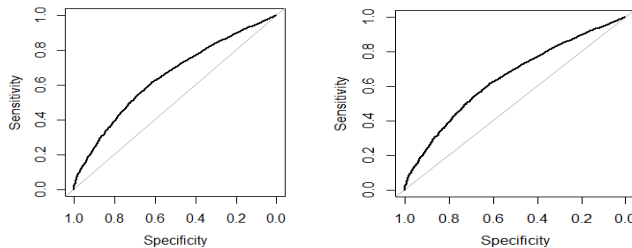
Figure 2: ROC curve from logistic regression model (left) and neural network model (right)
