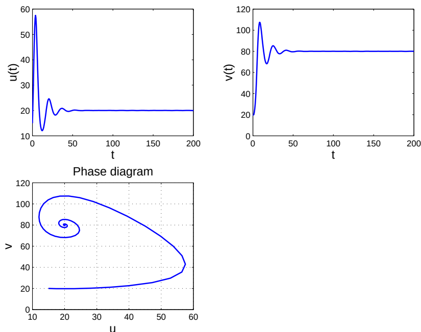
Figure 1: Stability of the capital-labour equilibrium E^* .
