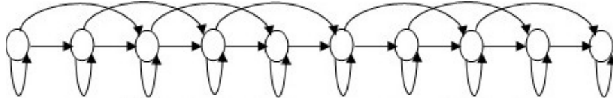
Figure 7: A 10-state Left-To-right Hidden Markov Model used to model Yorùbá alphabet
