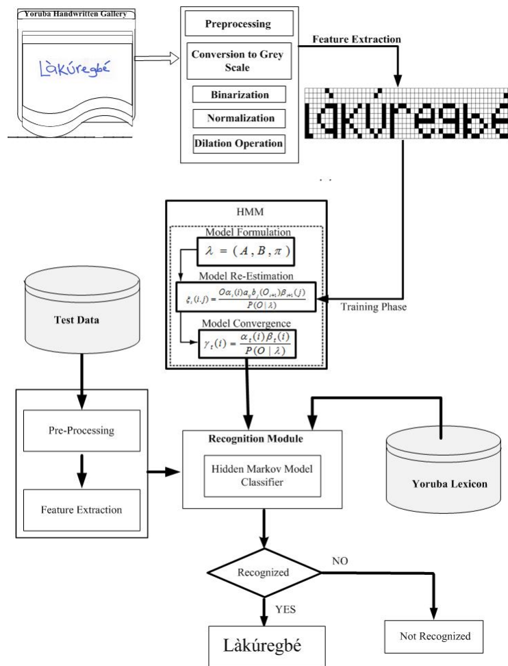
Figure 1: The framework architecture of the Recognition System
