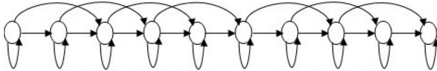
Figure 7: A 10-state Left-To-right Hidden Markov Model used to model Yorùbá alphabet
