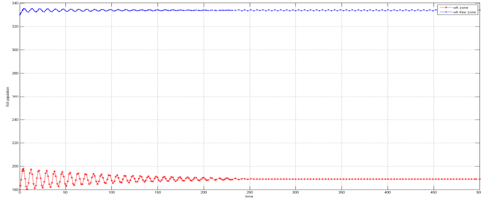
Fig.2.Stable variation of the population for \tau = 1.53
