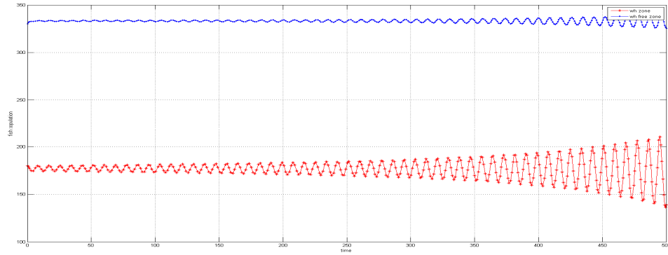
Fig.5.Unstable variation of the fish population for \tau = 1.495
