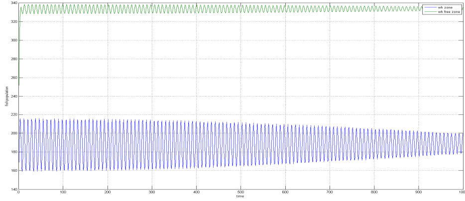
Fig.3.Unstable variation of the fish population for \tau = 1.549
