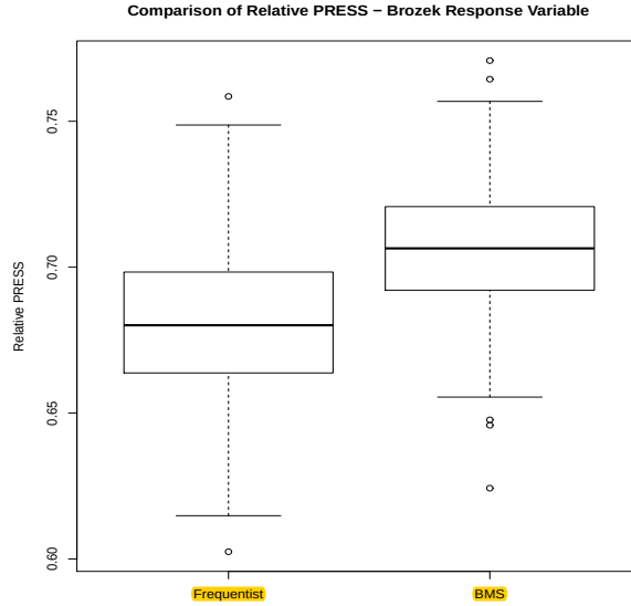
FIG 16. Comparison of Relative PRESS
