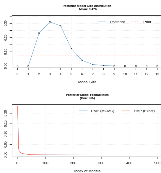
FIG 13. Optimal Model Size - Bayesian PIP Approach
