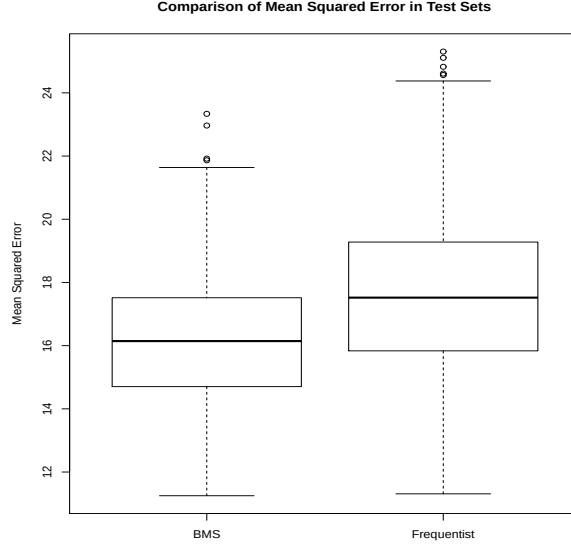
FIG 17. Figure: Comparison of MSE
