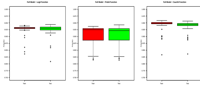
FIG 2. Comparative Boxplots of Training/Testing Accuracies - Logit (Left); Probit (Center); Cauchit (Right)
