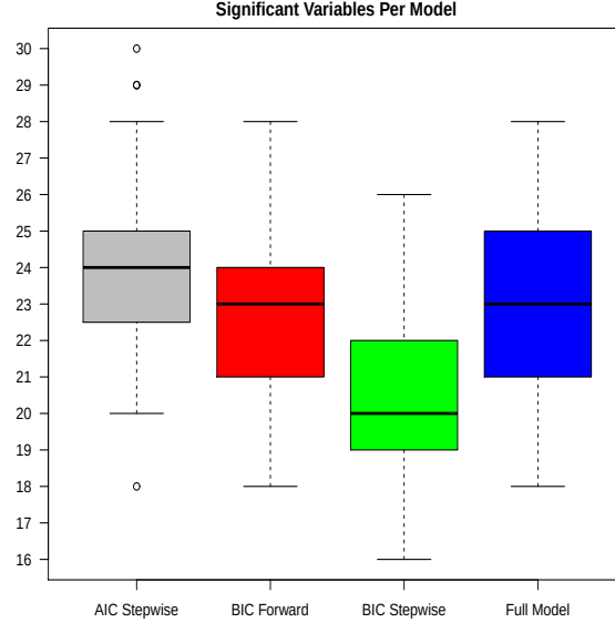
FIG 3. Number of Variables Deemed Significant in Replications
