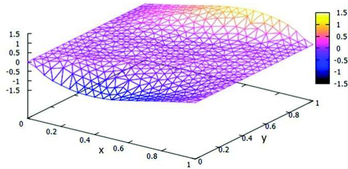
Figure 4: Elasticity model under constraint \varepsilon(u)w = 3w with w = (0; 1)
