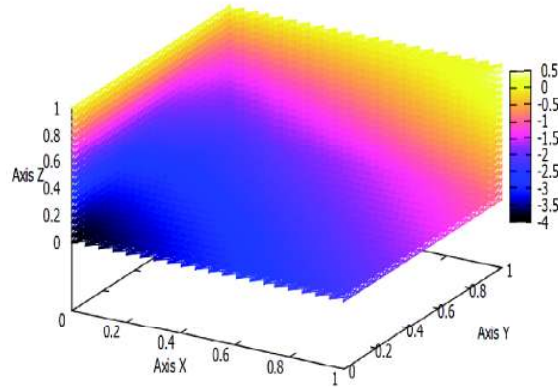
Figure 8: Elasticity model under constraint \varepsilon(u)w = 3w with w = (1; 1; 1)
