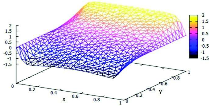
Figure 1: Poisson model under constraint, with \nabla_{uw} = 0 and w = (0; 1)
