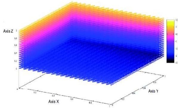
Figure 7: Elasticity model under constraint \varepsilon(u)w = 3w with w = (0; 0; 1)
