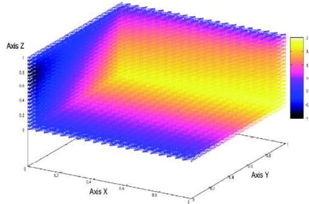
Figure 5: Elasticity model under constraint \varepsilon(u)w = 3w with w = (0; 1; 0)
