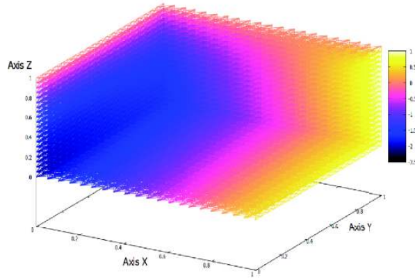
Figure 6: Elasticity model under constraint \varepsilon(u)w = 3w with w = (1; 0; 0)
