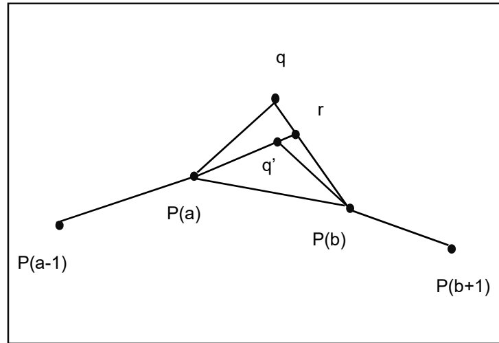
Fig. 18 Triangle (P(a), q, P(b)) . b is the next item number of a in P which is circular.
