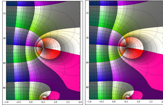
Figure 5: Sudden change of configuration in a neighborhood of a double zero.
