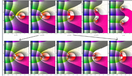
Figure 3: Double zero obtained by trial and error for \tau = 0.34375
