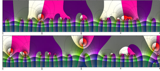
Figure 2: S_k^{(0)} \cap S_k^{(1)} contain roughly the same number of zeros
