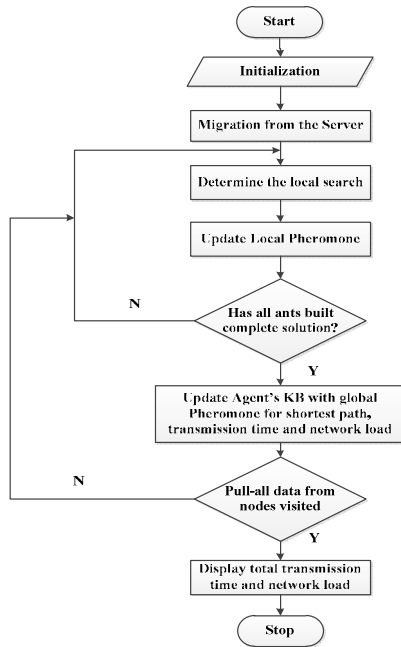
194 Fig. 1: Flowchart of the Developed migration pattern for the pull-all data strategy.
