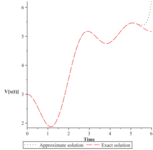
Figure 10: Variance approximation solution for the HAM with n = 18 . For A \sim U(\alpha = 0, \beta = 2) .
