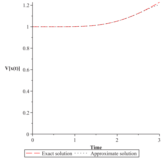
Figure 8: Variance approximation solution for the HAM with n = 18 . For A \sim U(\alpha = 0, \beta = 1) .
