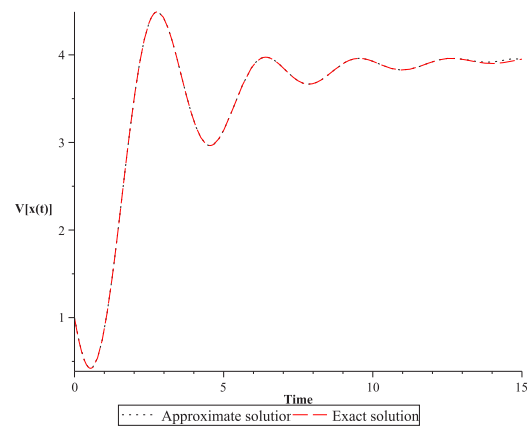
Figure 2: Variance approximation solution for the HAM with n = 18 . For A^2 \sim Be(\alpha = 2, \beta = 1) .
