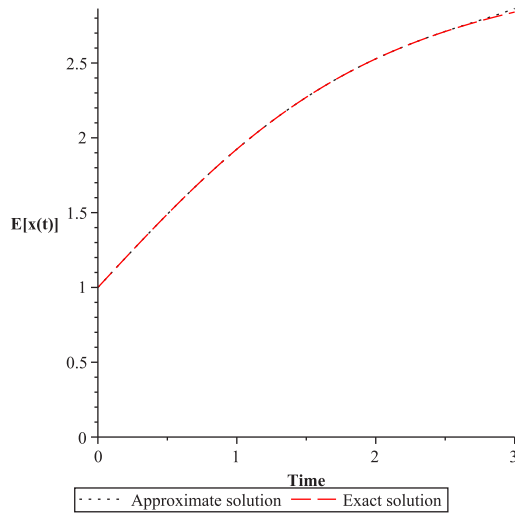
Figure 7: Expectation approximation solution for the HAM with n = 18 . For A \sim U(\alpha = 0, \beta = 1) .
