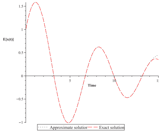
Figure 1: Expectation approximation solution for the HAM with n = 18 . For A^2 \sim Be(\alpha = 2, \beta = 1) .
