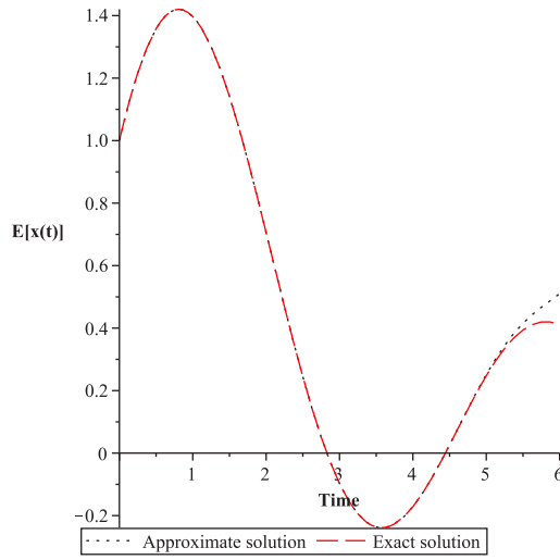
Figure 9: Expectation approximation solution for the HAM with n = 18 . For A \sim U(\alpha = 0, \beta = 2) .
