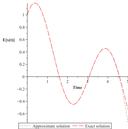
Figure 11: Expectation approximation solution for the HAM with n = 18 . For A \sim U(\alpha = 1, \beta = 2) .
