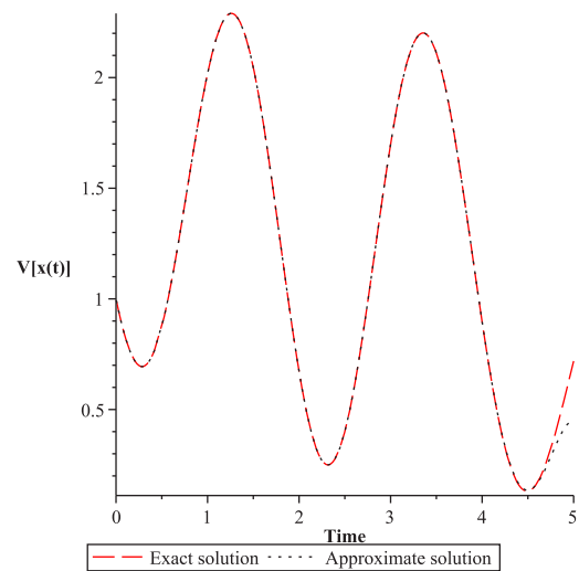
Figure 12: Variance approximation solution for the HAM with n = 18 . For A \sim U(\alpha = 1, \beta = 2) .
