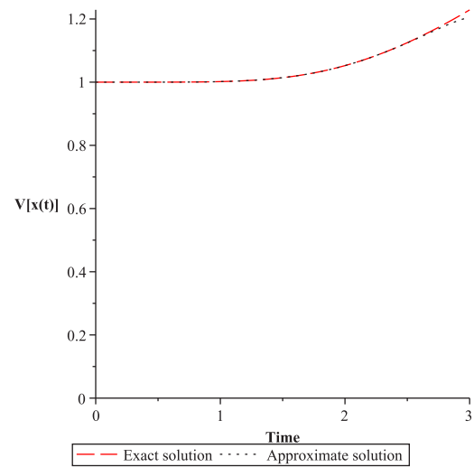
Figure 8: Variance approximation solution from the HAM with n = 18 . For A \sim U(\alpha = 0, \beta = 1) .
