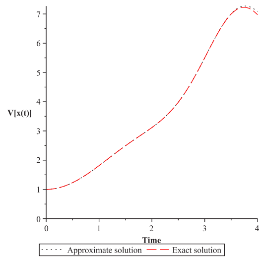
Figure 4: Variance approximation solution for the HAM with n = 18 . For A \sim Be(\alpha = 2, \beta = 3) .
