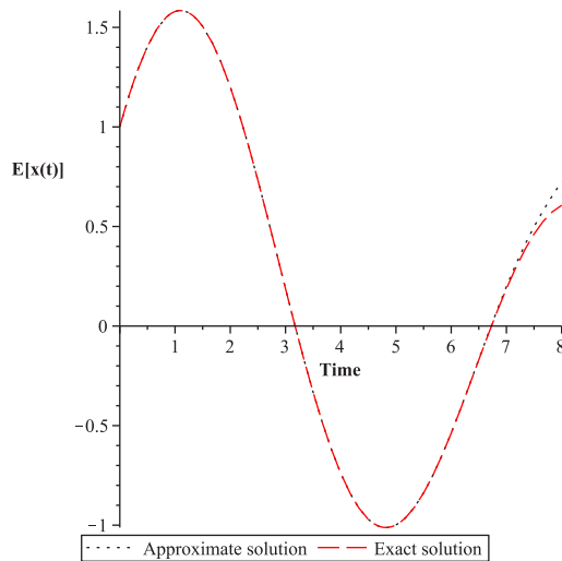
Figure 1: Expectation approximation solution for the HAM with n = 18 . For A^2 \sim Be(\alpha = 2, \beta = 1) .
