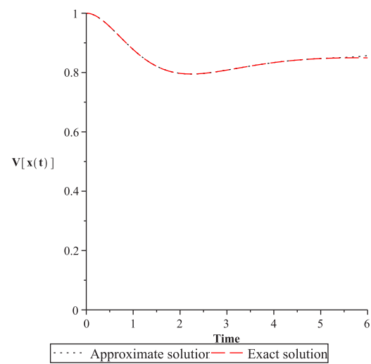
Figure 6: Variance approximation solution for the HAM with n = 18 . For A \sim Be(\alpha = 2, \beta = 1) .
