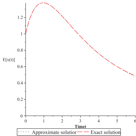
Figure 5: Expectation approximation solution for the HAM with n = 18 . For A \sim Be(\alpha = 2, \beta = 1) .
