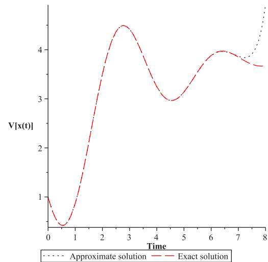
Figure 2: Variance approximation solution for the HAM with n = 18 . For A^2 \sim Be(\alpha = 2, \beta = 1) .
