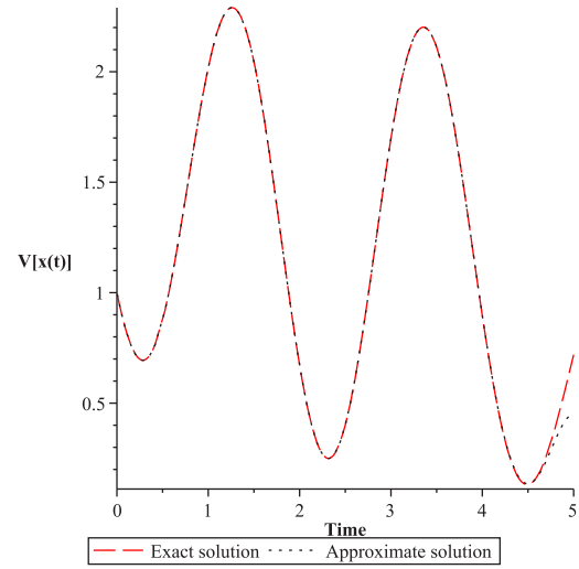
Figure 12: Variance approximation solution from the HAM with n = 18 . For A \sim U(\alpha = 1, \beta = 2) .
