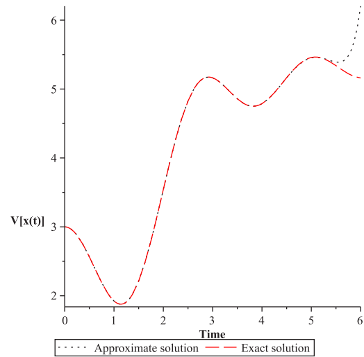
Figure 10: Variance approximation solution from the HAM with n = 18 . For A \sim U(\alpha = 0, \beta = 2) .
