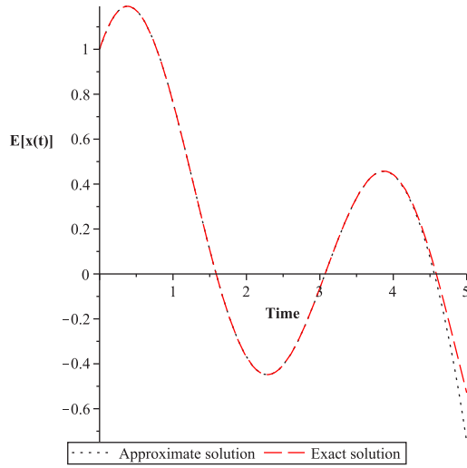
Figure 11: Expectation approximation solution from the HAM with n = 18 . For A \sim U(\alpha = 1, \beta = 2) .
