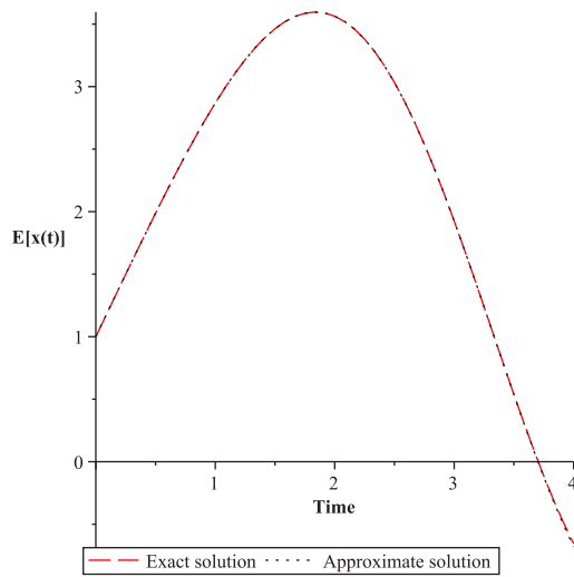
Figure 3: Expectation approximation solution for the HAM with n = 18 . For A \sim Be(\alpha = 2, \beta = 3) .
