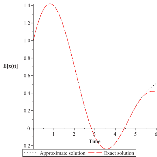
Figure 9: Expectation approximation solution from the HAM with n = 18 . For A \sim U(\alpha = 0, \beta = 2) .
