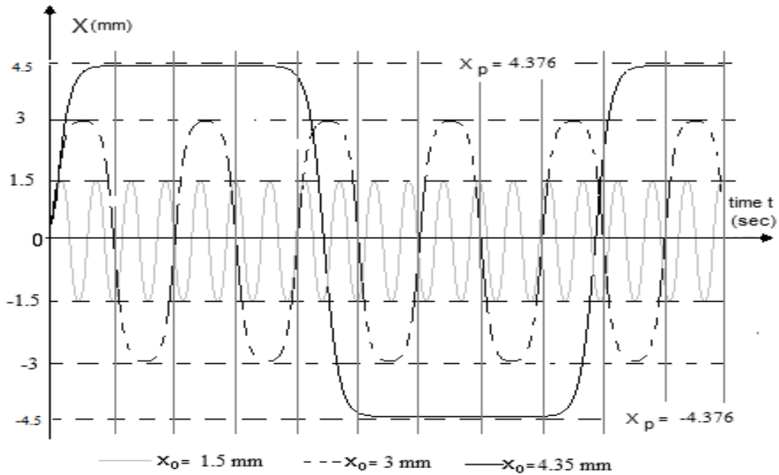
Figure 3. Graph of G_n function, depending on starting position
