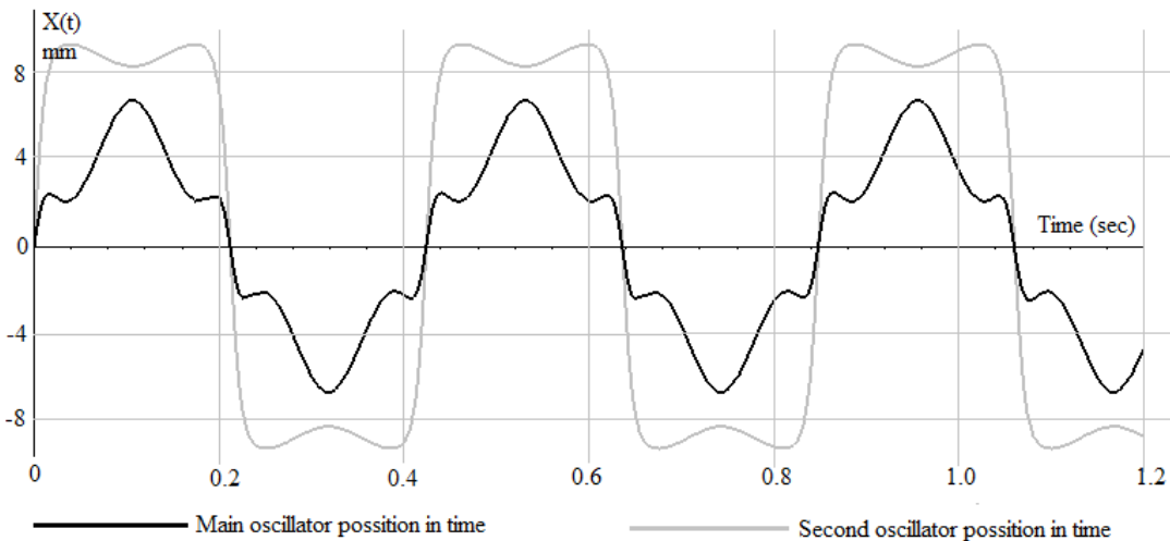
Figure 8. Graph for given physical system and starting condition e.
