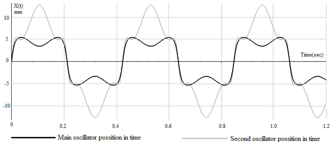
Figure 4. Graph for the given physical system and starting conditions a.
