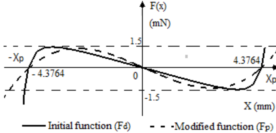
Figure 2. The graph of ( F_p , F_d ) functions, with the same roots and the same intergraphic area.
