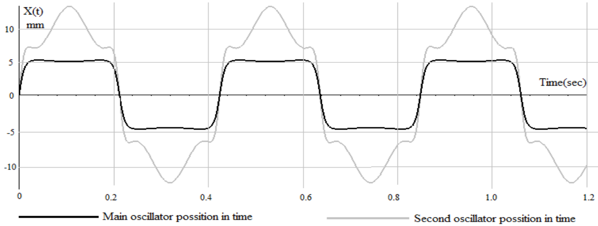
Figure 5. Graph for given physical system and starting conditions b.
