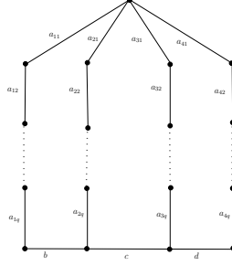
FIGURE 1. A general 4_q -fan
