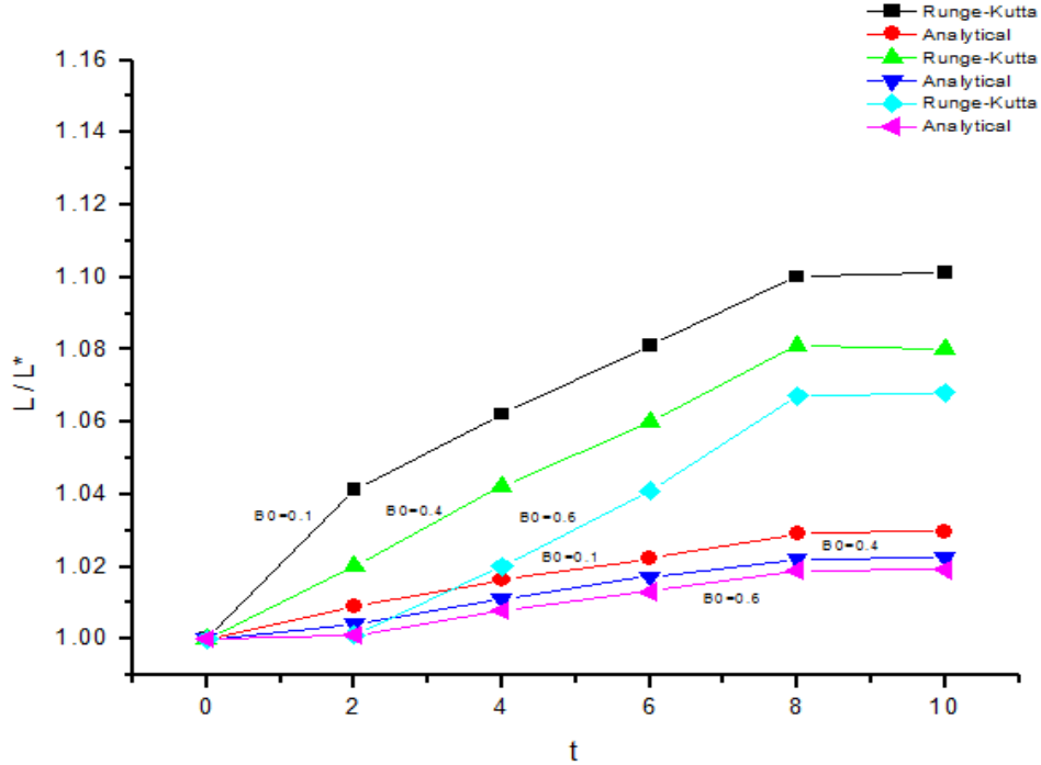
Figure 1:Non-equilibrium effect on the length of a saw-tooth profile for plane wave
