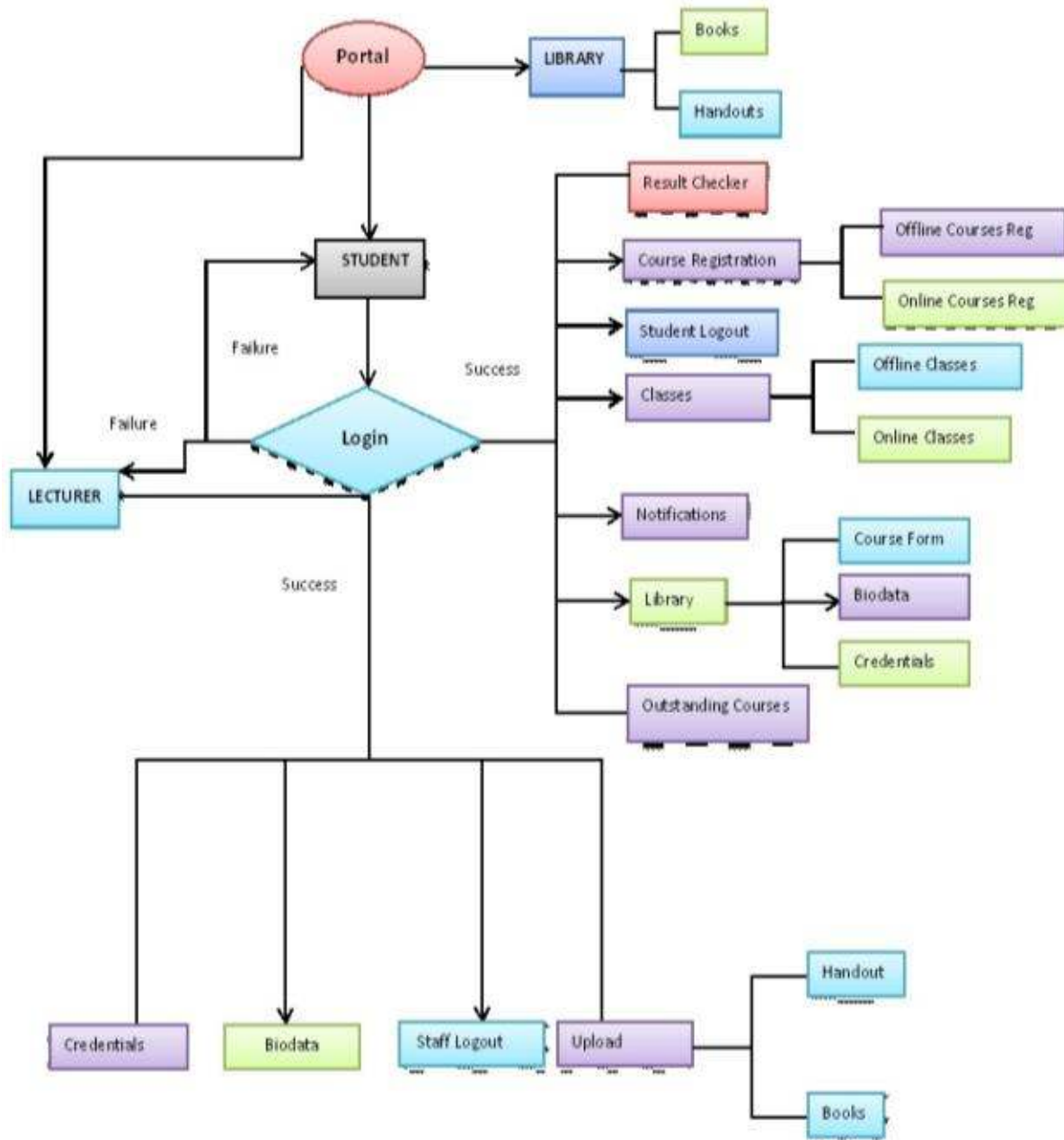
Fig. 4: The DFD of the Portal System
