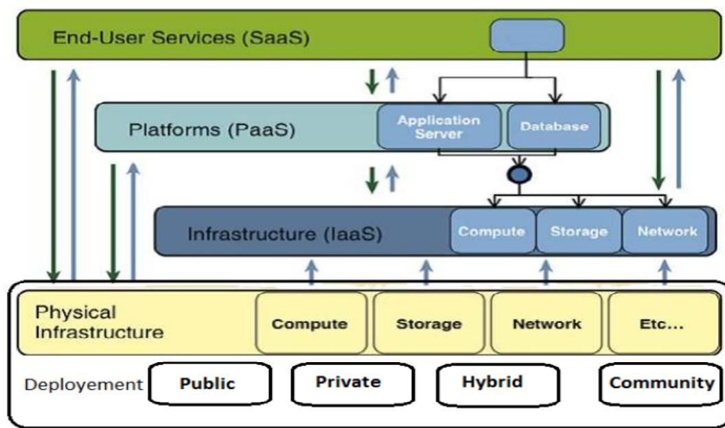
Fig. 1: Cloud Based Model
