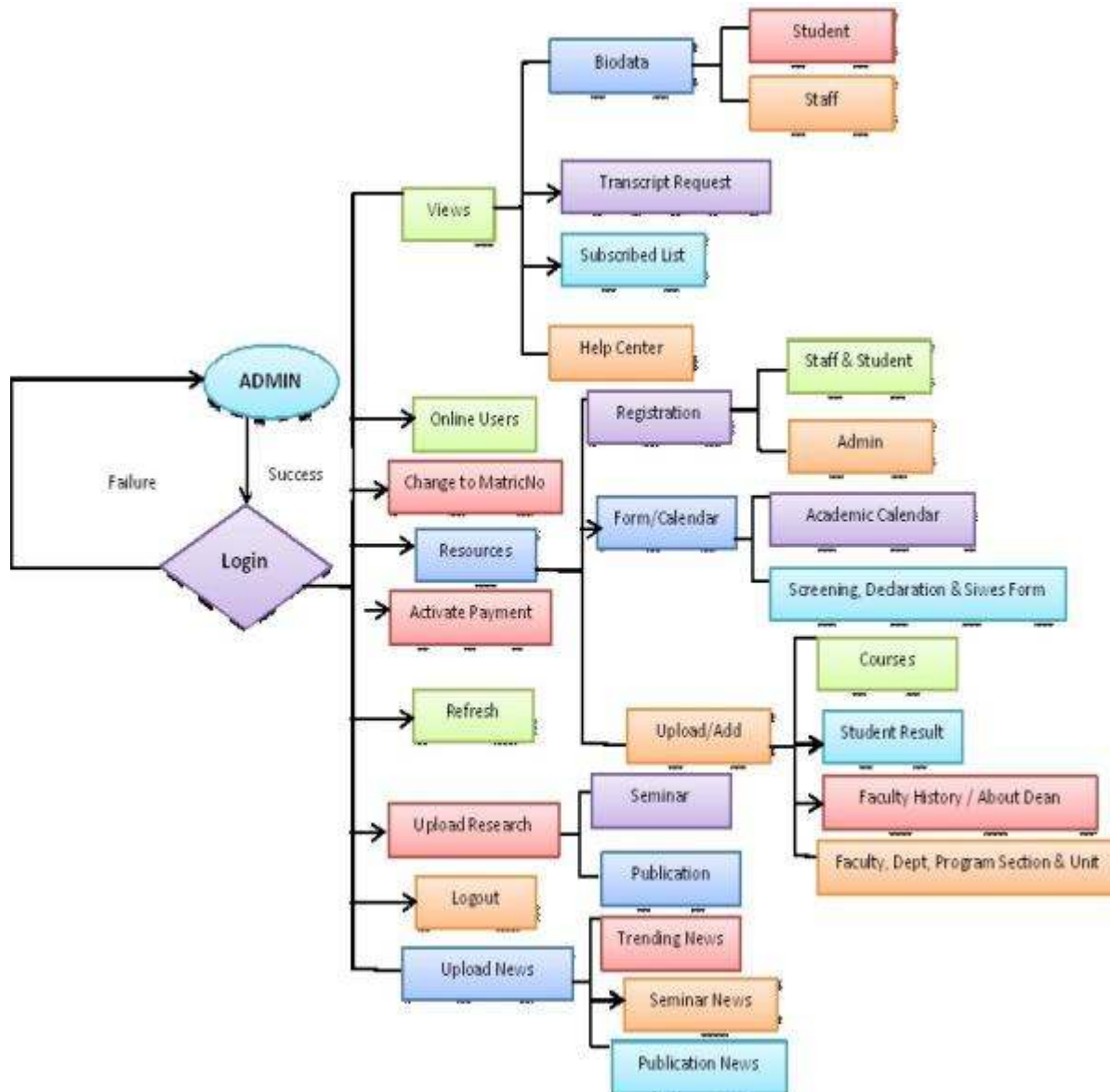
Fig. 5: The DFD of the Admin System
