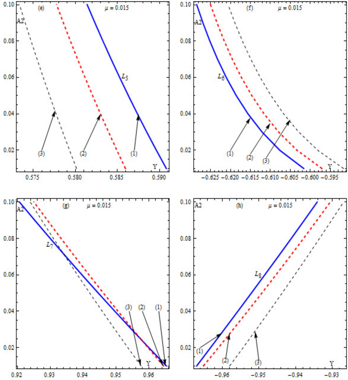
Fig.2.2 Frames (a) to (h). The positions of the equilibrium points L_i, i = 1, \dots, 8 in the (y, A_2) plane as the oblateness factor varies for fixed values of triaxial factor: (1) \sigma_1 = 2.284 \times 10^{-12}, \sigma_2 = 1.141 \times 10^{-12} , (2) \sigma_1 = 0.025, \sigma_2 = 0.015 and (3) \sigma_1 = 0.085, \sigma_2 = 0.065 . The mass distribution is m_1 = 0.97 and m_2 = m_3 = \mu = 0.015 .
