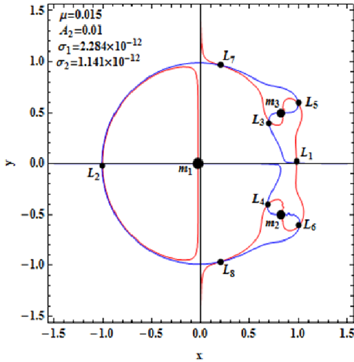
172 173 Fig.1. The positions of the equilibrium points L_i , i=1,\dots,8 of the problem for \mu = 0.015 , 174 \sigma_1 = 2.284 \times 10^{-12} , \sigma_2 = 1.141 \times 10^{-12} and A_2 = 0.01 . The mass distribution is m_1 = 0.97 and 175 m_2 = m_3 = \mu = 0.015 . With large black points and small dots, we indicate the primary 176 bodies and equilibrium points of the problem correspondingly.
