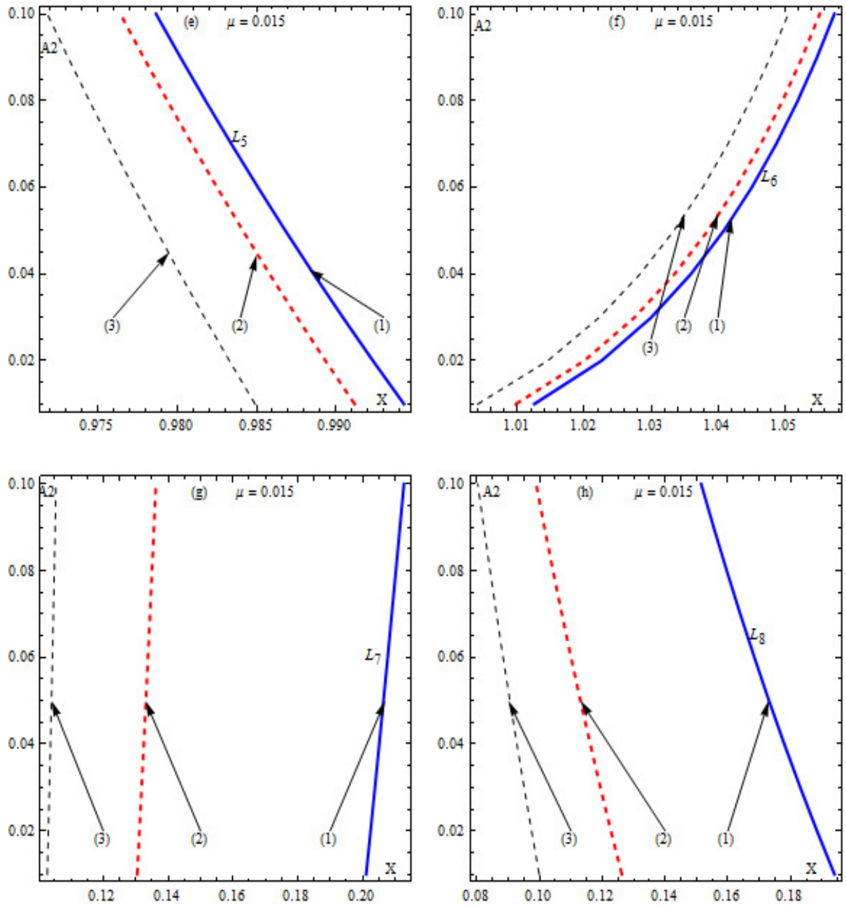
Fig.2.1 Frames (a) to (h). The positions of the equilibrium points L_i, i = 1, \dots, 8 in the (x, A_2) plane as the oblateness factor varies for fixed values of triaxial factor: (1) \sigma_1 = 2.284 \times 10^{-12}, \sigma_2 = 1.141 \times 10^{-12} , (2) \sigma_1 = 0.025, \sigma_2 = 0.015 and (3) \sigma_1 = 0.085, \sigma_2 = 0.065 . The mass distribution is m_1 = 0.97 and m_2 = m_3 = \mu = 0.015 .
