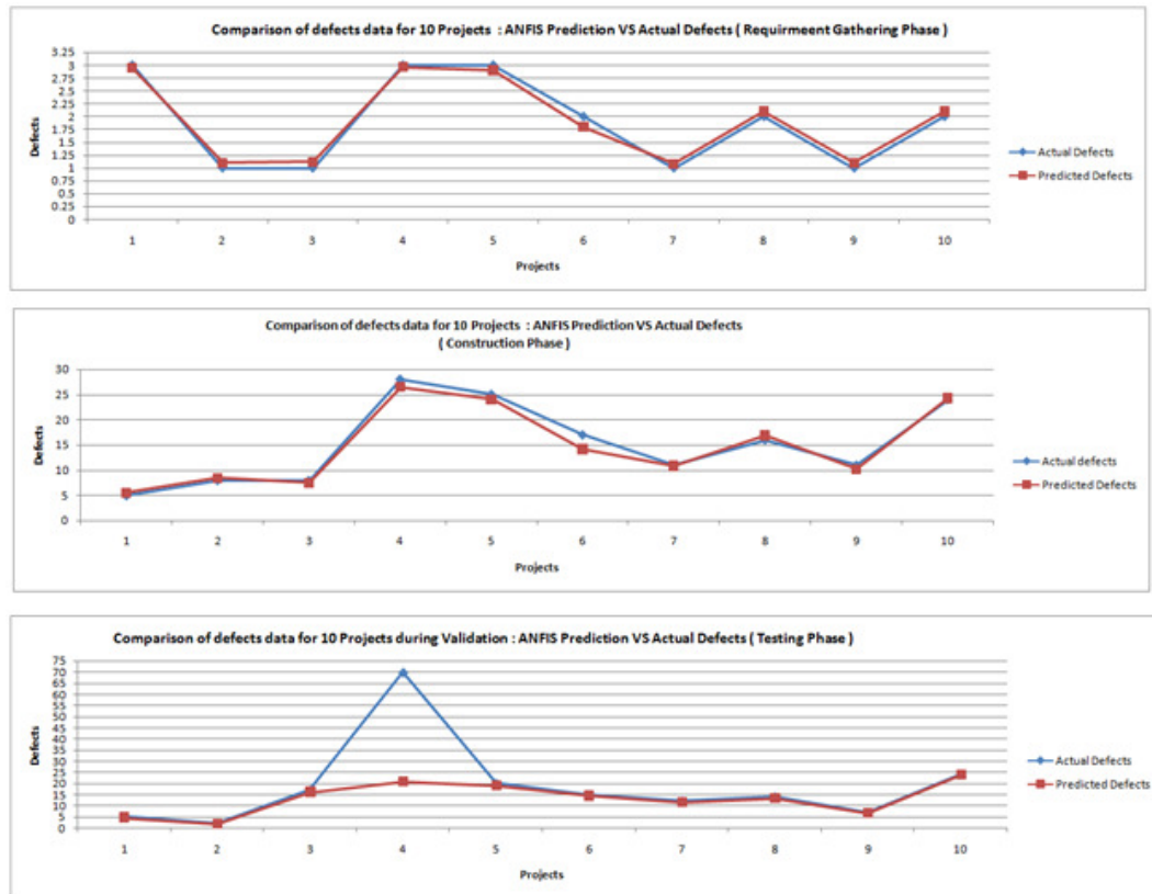
Figure 8 Comparative trend of defects predicted by ANFIS Vs Actual Defects
