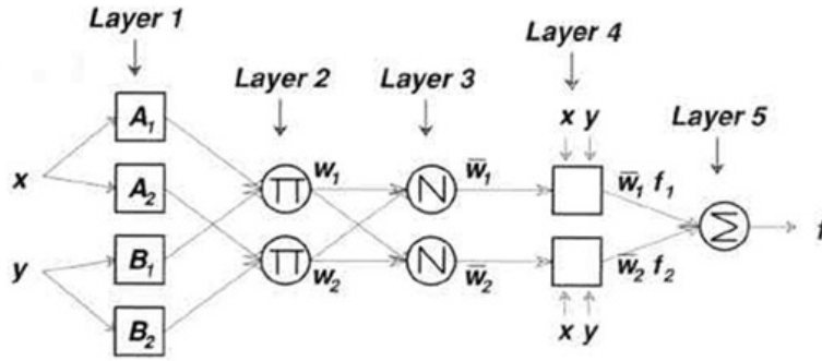
Figure 2 Equivalent ANFIS architecture ( Jang, 1993)
