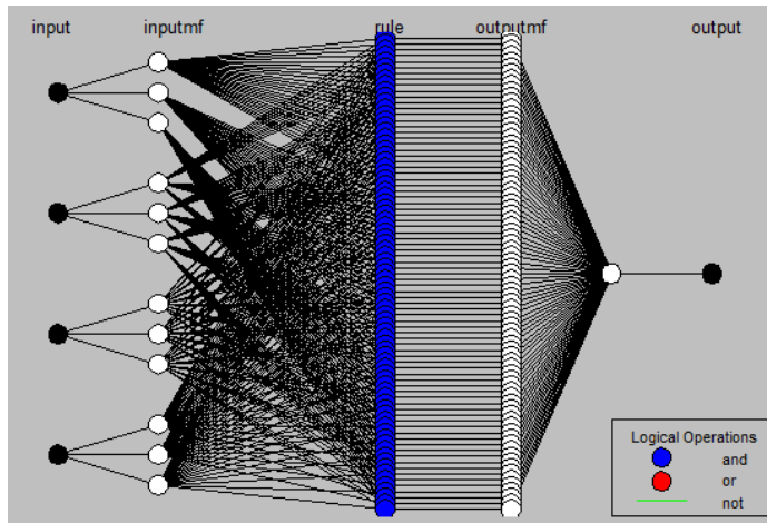
Figure 3 ANFIS Structure for Requirement Gathering Phase with four inputs
