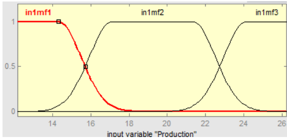
Figure 5 Membership Functions for inputs (Production effort)
