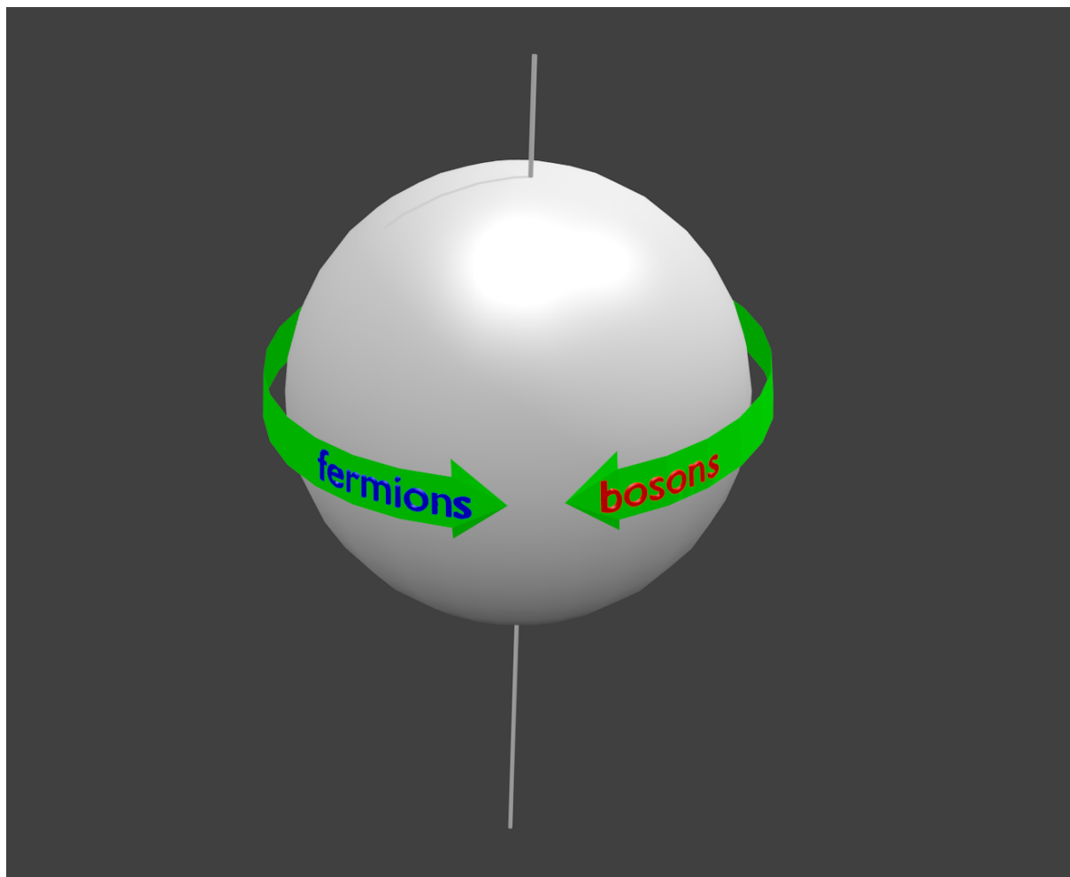
Figure 1: Schematic view of a free particle bound state, in which the rotation of fermions is counterbalanced by bosons.
