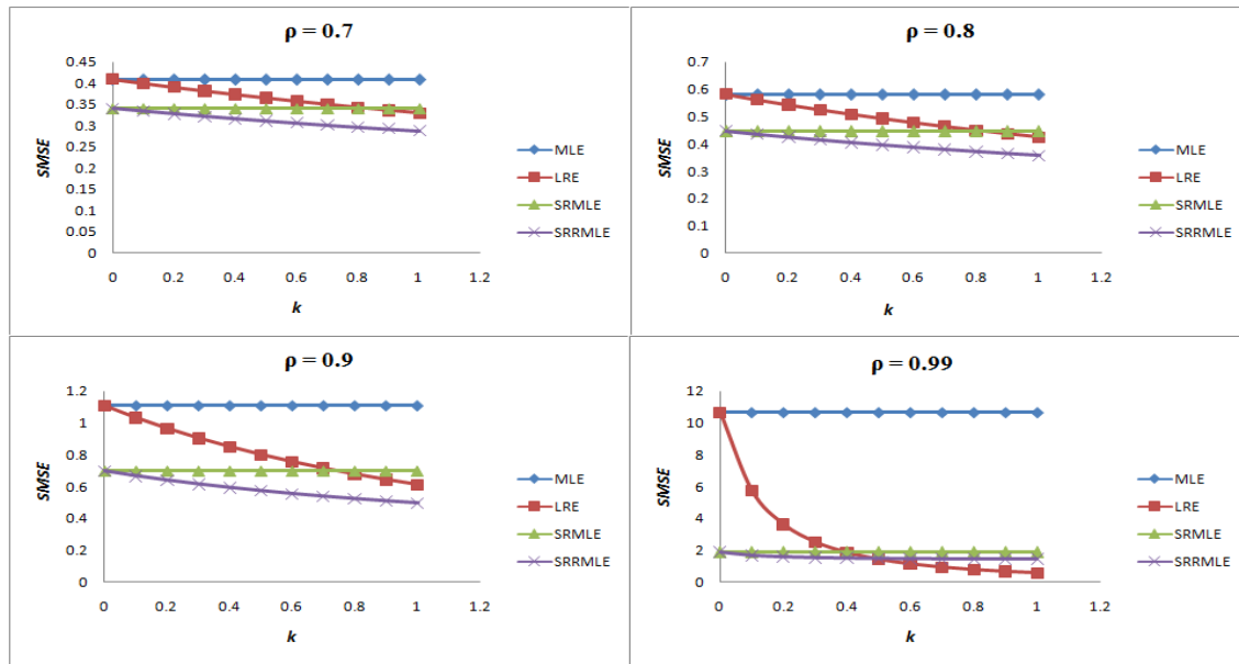
Figure 5.4: Estimated SMSE values for MLE, LRE, SRMLE and SRRMLE for n = 100
