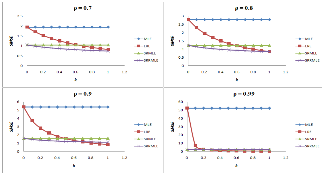
Figure 5.1: Estimated SMSE values for MLE, LRE, SRMLE and SRRMLE for n = 25
