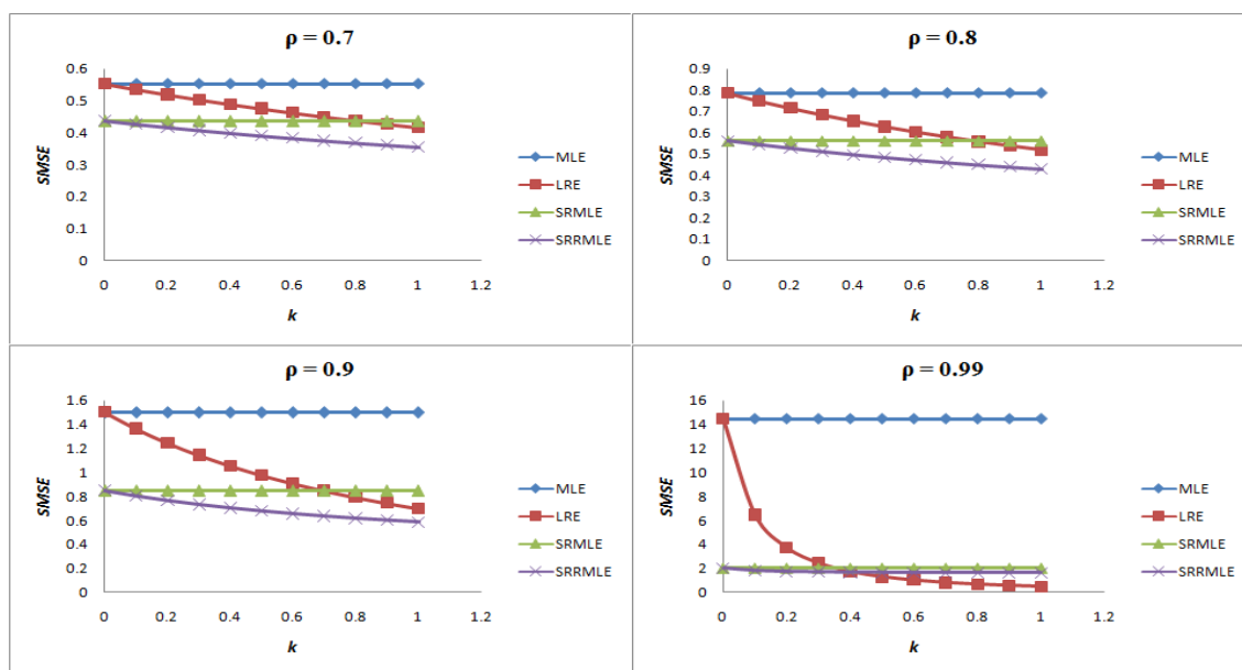
Figure 5.3: Estimated SMSE values for MLE, LRE, SRMLE and SRRMLE for n = 75
