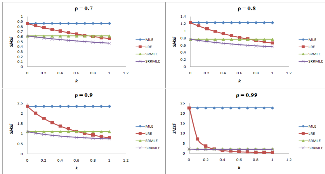
Figure 5.2: Estimated SMSE values for MLE, LRE, SRMLE and SRRMLE for n = 50
