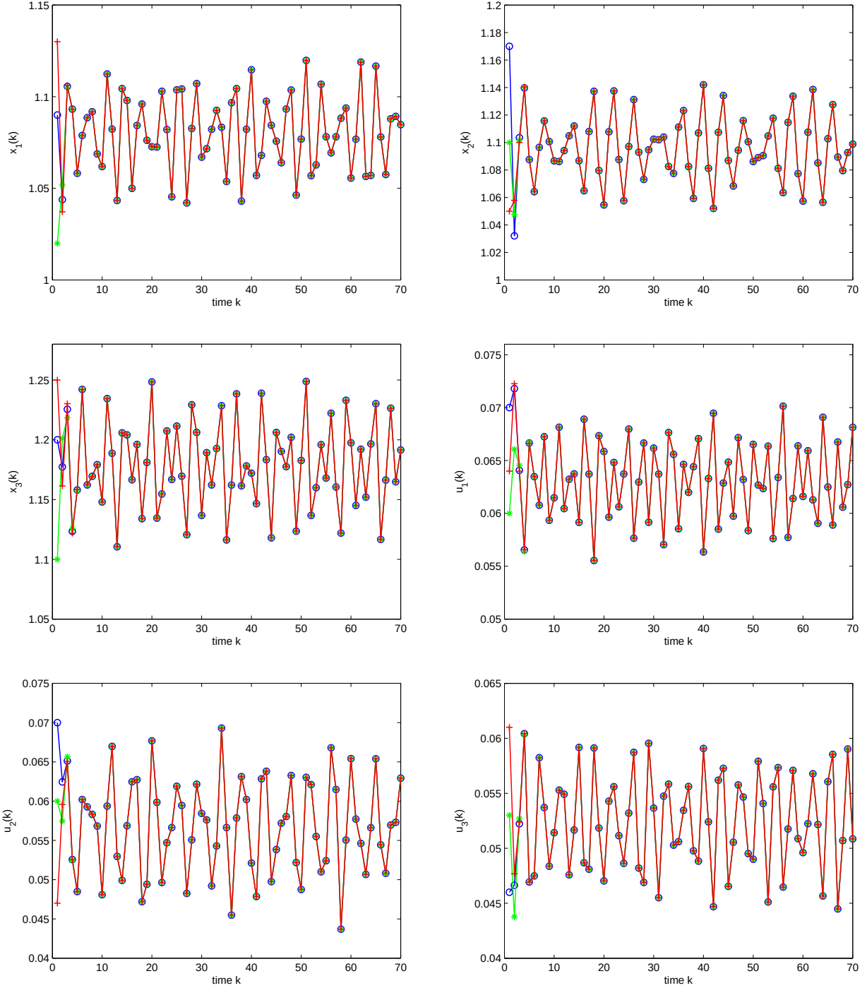
FIGURE1: Dynamic behavior of positive almost periodic solution (x_1(k), x_2(k), x_3(k), u_1(k), u_2(k), u_3(k)) of system (5.1) with the three initial conditions (1.02, 1.1, 1.1, 0.06, 0.06, 0.053) , (1.09, 1.17, 1.2, 0.07, 0.07, 0.046) and (1.13, 1.05, 1.25, 0.064, 0.047, 0.061) for k \in [1, 70] , respectively.
