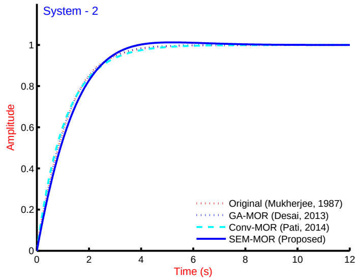
Figure 2: Step response of original system as in Eqn. 3.28, ROM as in Eqns. 3.29 - 3.30 and proposed ROM using Stability equation method as in Eqn. 3.35.
