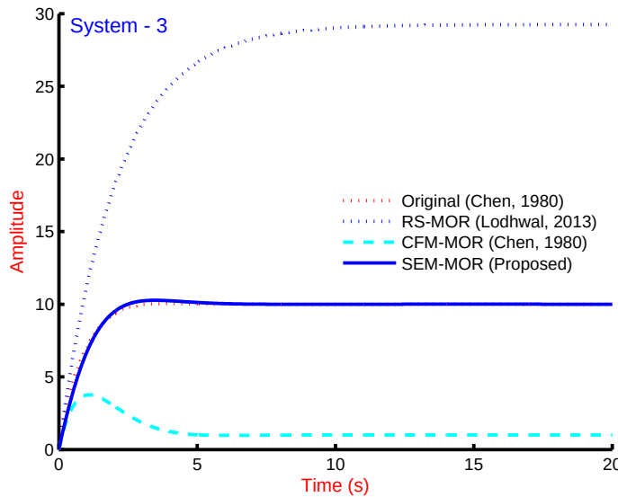
Figure 3: Step response of original system as in Eqn. 3.36, ROM as in Eqns. 3.37 - 3.38 and proposed ROM using Stability equation method as in Eqn. 3.43.
