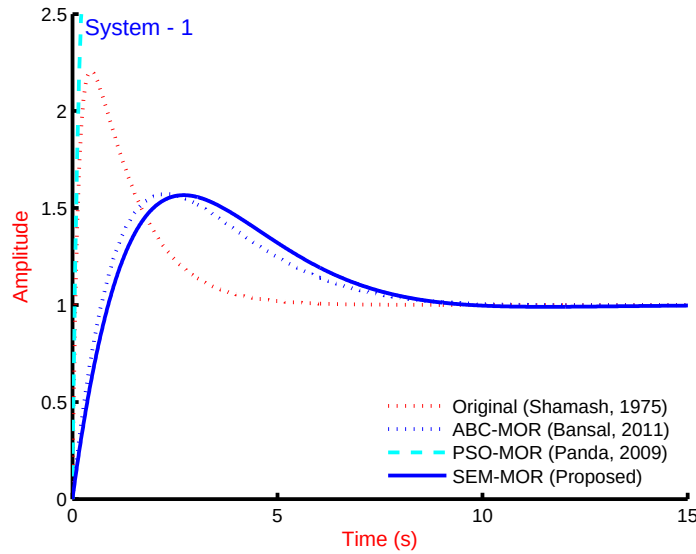
Figure 1: Step response of original system as in Eqn. 3.1, ROM as in Eqns. 3.2 - 3.3 and proposed ROM using Stability equation method as in Eqn. 3.27.
