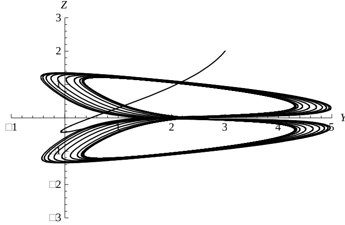
Figure 10: Y-Z Phase portrait using 10-term MLADM on \Delta t = 0.01 for d = 2 , e = -0.1 and f = 1.6 , \alpha = 1 .
