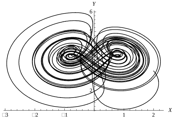
Figure 2: X-Y Phase portrait using 10-term MLADM on \Delta t = 0.01 for d = 3, e = 0.1 and f = 1, \alpha = 1 .
