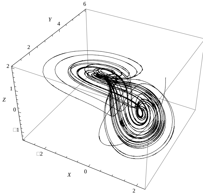
181 182 Figure 1: X-Y-Z Phase portrait using 10-term MLADM on \Delta t = 0.01 for d = 3, 183 e = 0.1 and f = 1 .
