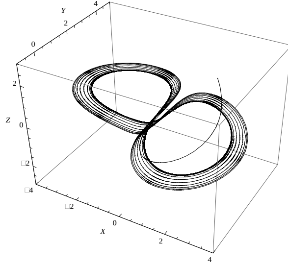
225 Figure 8: X-Y-Z Phase portrait using 10-term MLADM on \Delta t = 0.01 for d = 2 , e = -0.1 226 and f = 1.6 , \alpha = 1 .
