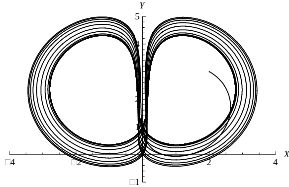
229 Figure 9: X-Y Phase portrait using 10-term MLADM on \Delta t = 0.01 for d = 2 , e = -0.1 230 and f = 1.6 , \alpha = 1 .
