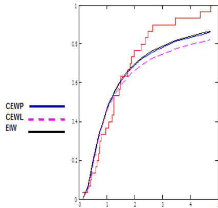
Figure (13): Estimated cumulative densities for the third data
