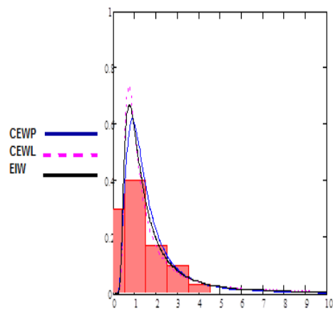
Figure(12): Estimated densities for the second data
