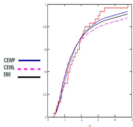
Figure (11): Estimated cumulative densities for the second data
