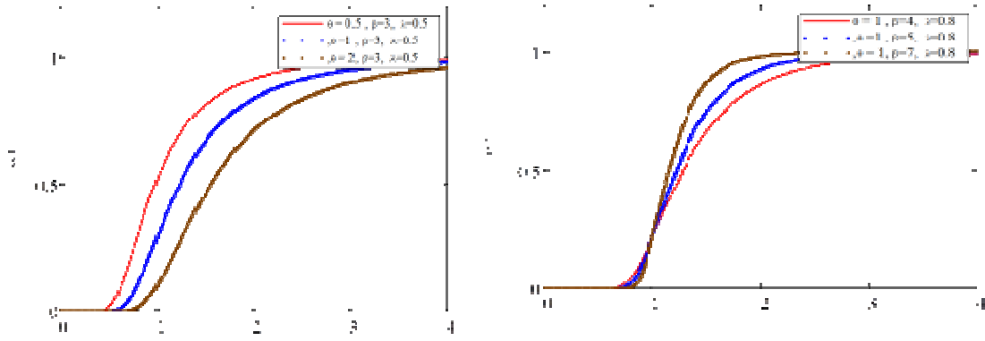
Figure (6): Plots of the cdf of the CEIWL for some parameter values
