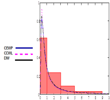
Figure (10): Estimated densities of models for the first data
