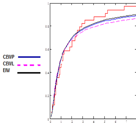
Figure (9) : Estimated cumulative densities for the first data
