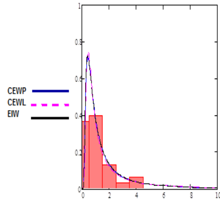
Figure (14): Estimated densities of the third data
