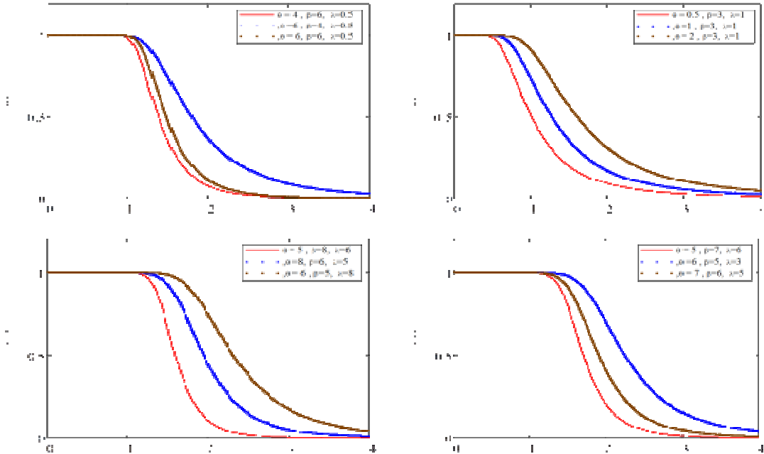
Figure (3): Plots of the CEIWP reliability functions for some parameter values
