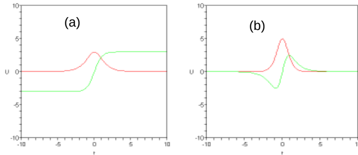
Fig. 1. Curves of |U_{11}| , |U_{12}| , |U_{21}| and |U_{22}| as a function of time; (a): the red curve indicates the profile of |U_{11}| for a=5 and \alpha=1 ; the green curve the profile of |U_{12}| for b=5 and \alpha=1 ; (b): the red curve indicates the profile of |U_{21}| for c=5 and \alpha=1 ; the green curve gives the profile of |U_{22}| for d=5 and \alpha=1 ;
