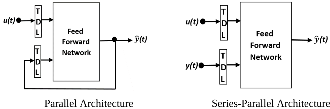
Figure (2.2) Architecture of NARX network.
