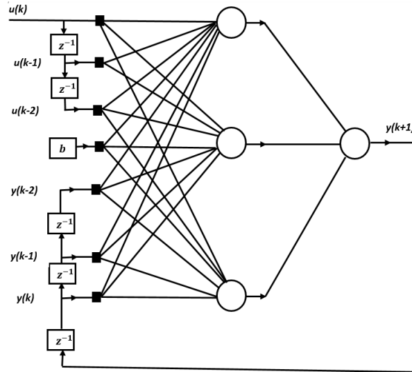
Figure(2.1):NARX model with tapped delay line at input.
