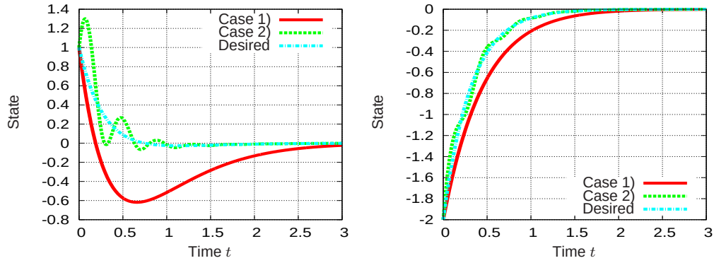
Figure 4: Time histories of the state x_1(t) : \Sigma_2^* (Left) and the state x_2(t) : \Sigma_2^* (Right)
