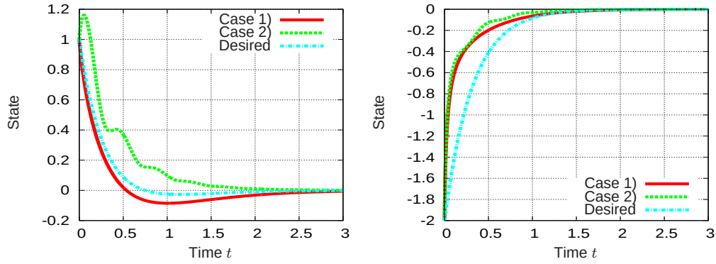
Figure 2: Time histories of the state x_1(t) : \Sigma_1^* (Left) and the state x_2(t) : \Sigma_1^* (Right)
