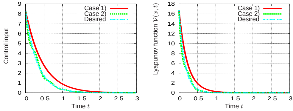
Figure 5: Time histories of the control input u(t) : \Sigma_2^* (Left) and the Lyapunov function \mathcal{V}(x, t) : \Sigma_2^* (Right)
