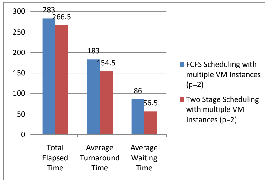
Fig. 2. Comparison of Performance Evaluation Metrics in different scheduling strategies.
