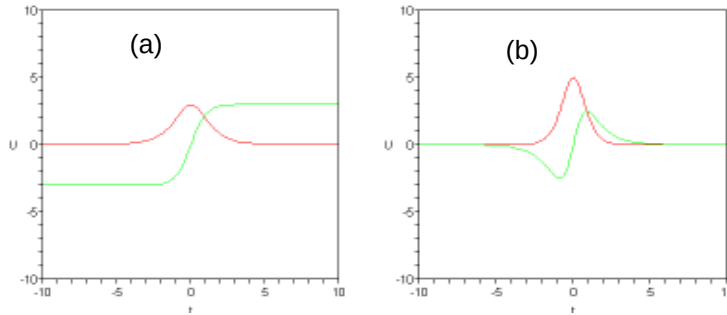
58 Fig. 1. Curves of |U_{11}| , |U_{12}| , |U_{21}| and |U_{22}| as a function of time; (a): the red curve indicates the 59 profile of |U_{11}| for a = 5 and \alpha = 1 ; the green curve the profile of |U_{12}| for b = 5 and \alpha = 1 ; 60 (b): the red curve indicates the profile of |U_{21}| for c = 5 and \alpha = 1 ; the green curve gives the 61 profile of |U_{22}| for d = 5 and \alpha = 1 ; 62
