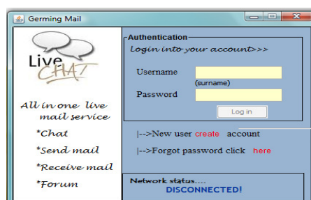
Figure 4: Login Interface
