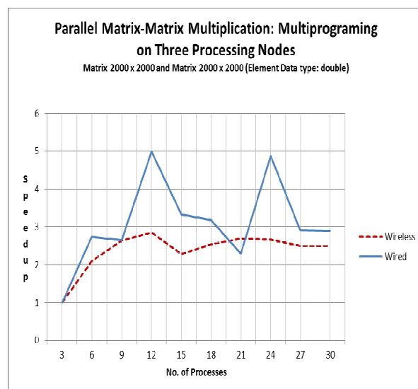
Figure 10 : Matri-Matrix Multiplication-Multiprogramming approach on Three Machines
