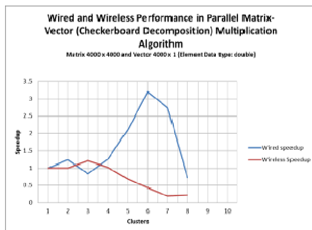
Figure 7 : Parallel Matrix-Vector Multiplication: Checkerboard decomposition speedup on wired and wireless
