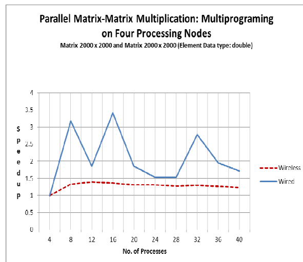
Figure 11: Matrix-Matrix Multiplication - Multiprogramming approach on Four machines
