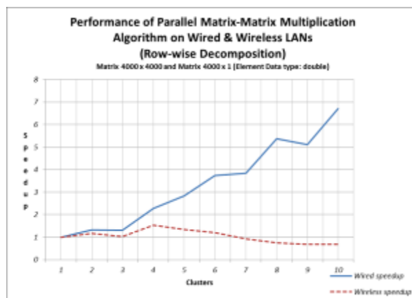
Figure 8 : Parallel Matrix-Matrix Multiplication Speedup on Wired and Wireless
