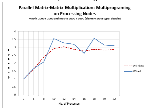
Figure 9: Matrix-Matrix Multiplication-Multiprogramming approach on Two machines
