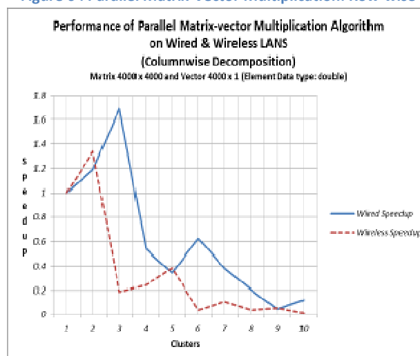
Figure 5: Matrix-Vector Multiplication (Column-wise Decomposition) Speedup on Wired and Wireless
