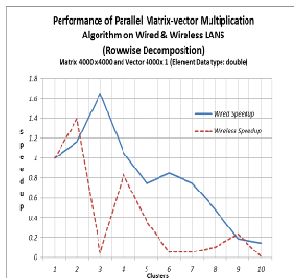
Figure 6 : Parallel Matrix-Vector Multiplication: Row-wise
