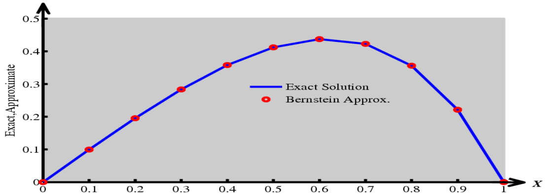
Fig. 2: Graphical representation of exact and approximate solutions of example 3
