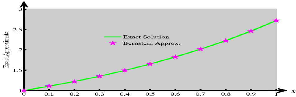
Fig. 3: Graphical representation of exact and approximate solutions of example 4
