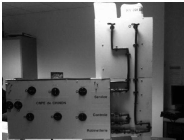
220 Fig. 1. Picture of the hydraulic mock-up: on the right, visible ducts and valves; on the 221 left, only valves are visible
