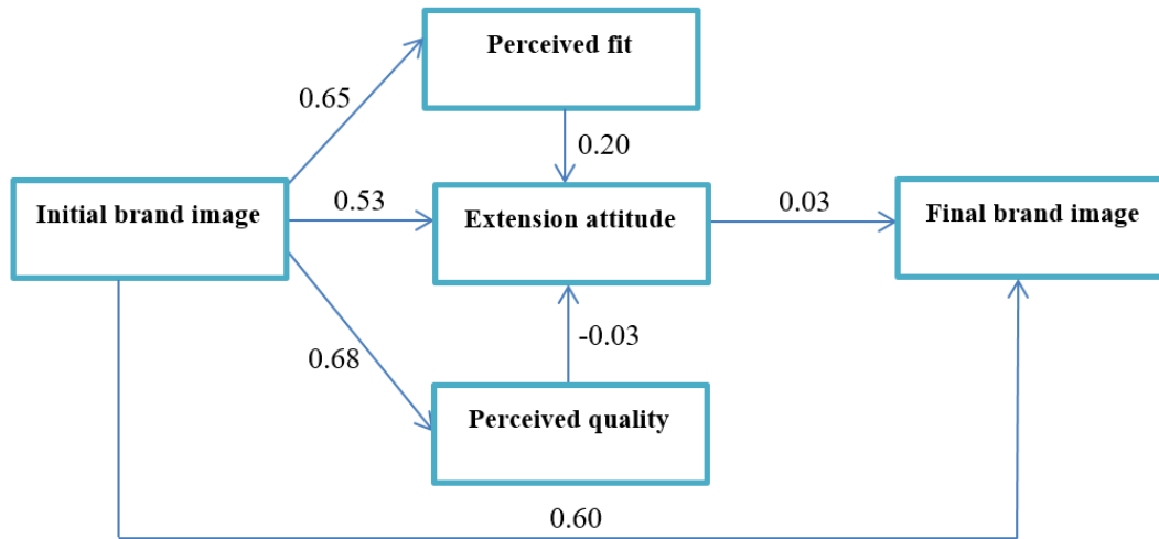
215 216 Figure. 2. Structural Equations Model 217
