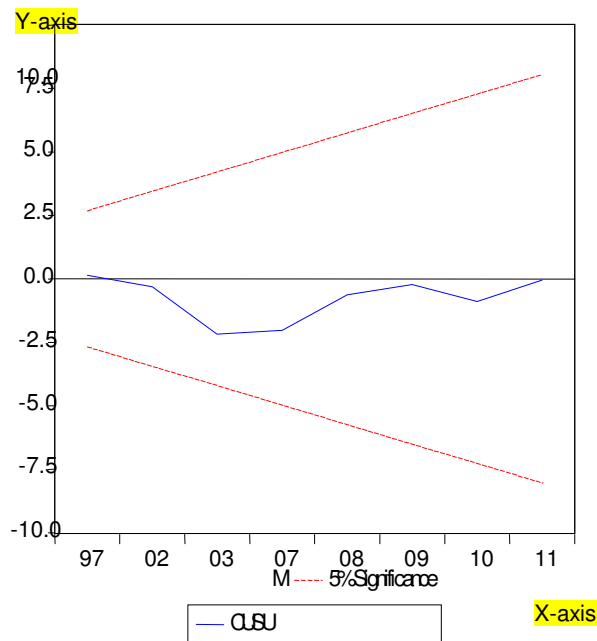
Figure 2: CUSUM Residual
