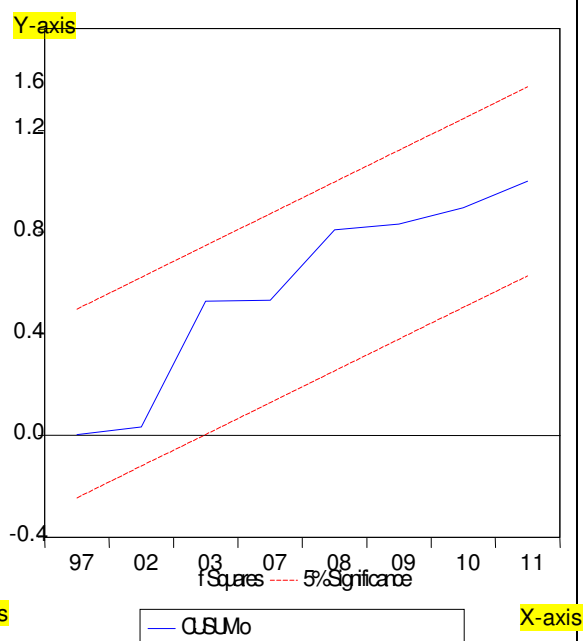
Figure 3: CUSUMsq Residual
