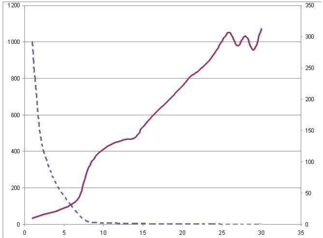
Figure 2. Dynamics of the output in case when the process of learning is described by Eq. (5) under t = 2, \dots, 7 and by Eq. (6) under t = 8, 9, \dots . Output in dependence on time is depicted by the red (unbroken) line. The blue (broken) line shows the endogenous change in parameter h_L .
