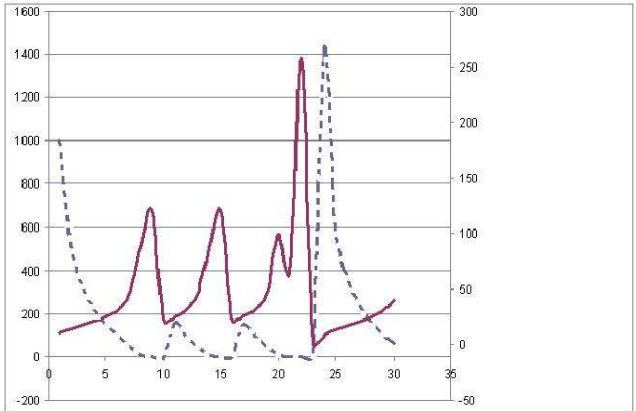
Figure 1. Dynamics of the output in case when the process of learning is described by Eq. (5) for all t = 2, 3, \dots . Output in dependence on time is depicted by the red (unbroken) line. The blue (broken) line shows the endogenous change in parameter h_L .
