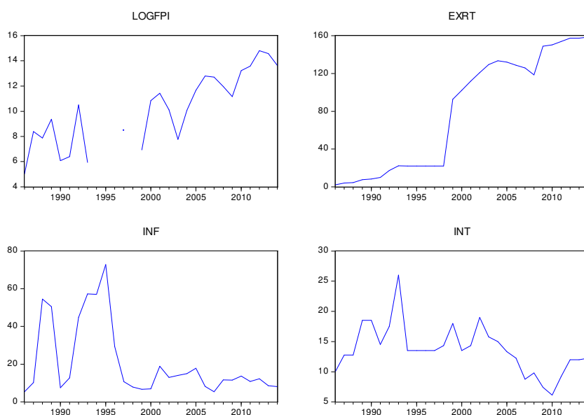
Fig. 4.1 Graphical Analysis of the logFPI, INT, INF and EXRT
