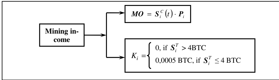
Picture 2. Income for i -indexed user in BTC network.
