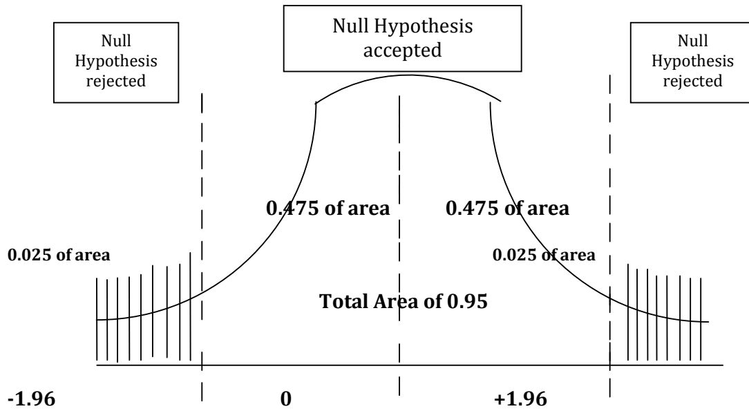
FIGURE 1: Two tailed Z-test( \alpha = 0.05 )
