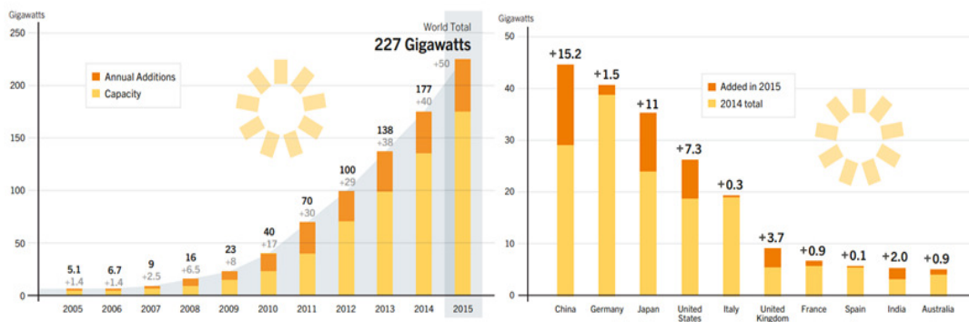
Fig. 5. Global Capacity of Photovoltaic Systems (a); Capacity and Additions in 2015 (b) [31].
