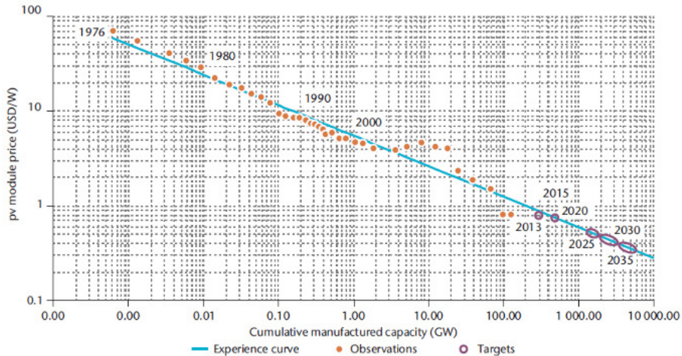
214 Fig. 4. Photovoltaic modules old prices and 2035 projection [21].
