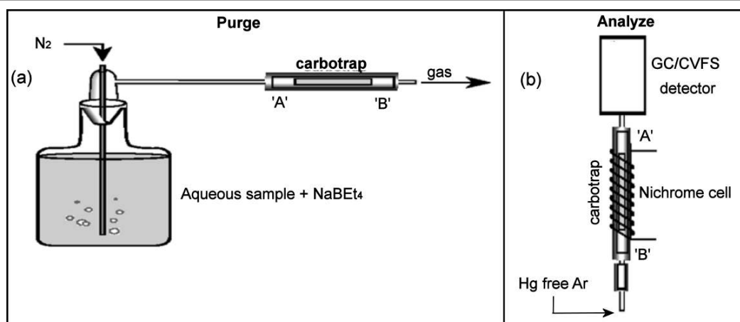
Fig. 6. Schematic diagram of bubbler setup and carbotrap® trap orientation 179 .
