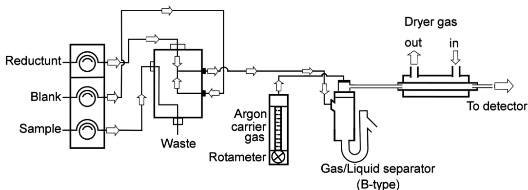
Fig. 5. Diagram of the mercury flow system. 177
