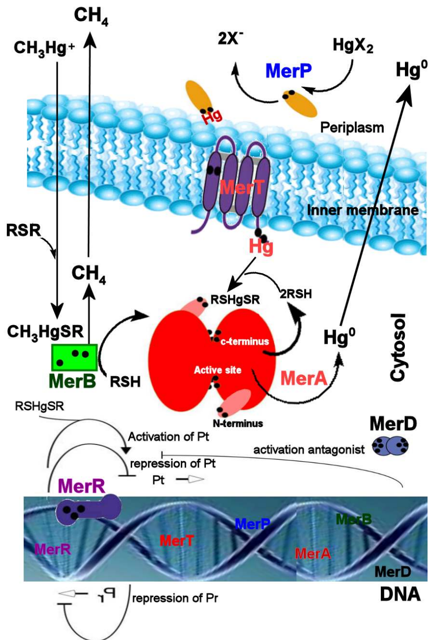
Fig. 3. Degradation/resistance of mercury by bacteria (see text for explanation and/or refer to Barkay et al for finer details). 11
