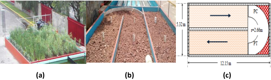
Fig 1: a). View Wetland with plants. b). Details of curve instead in channels. c). View curves shapes with slope
