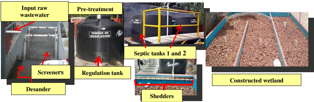
Fig. 2: Different parts of municipal wastewater treatment system by a constructed wetland.
