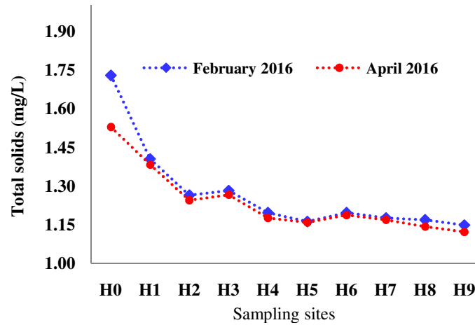
294 295 Fig. 10: TSS variation in wetland in two sampling periods
