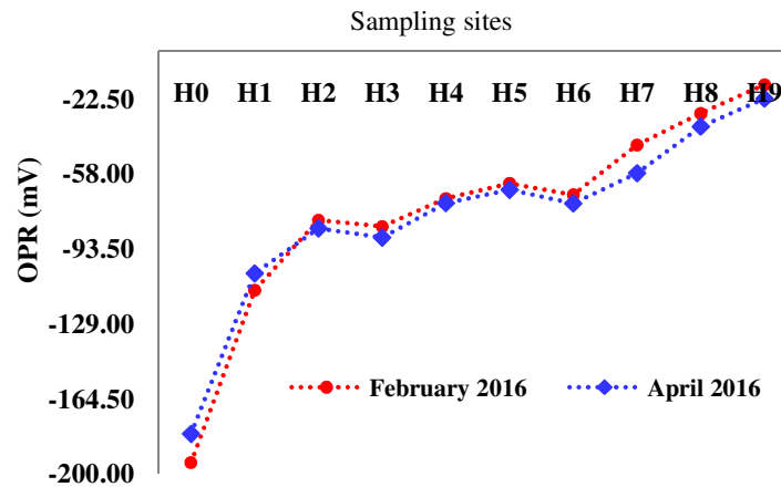
301 302 Fig. 11: OPR variation in wetland in two sampling periods
