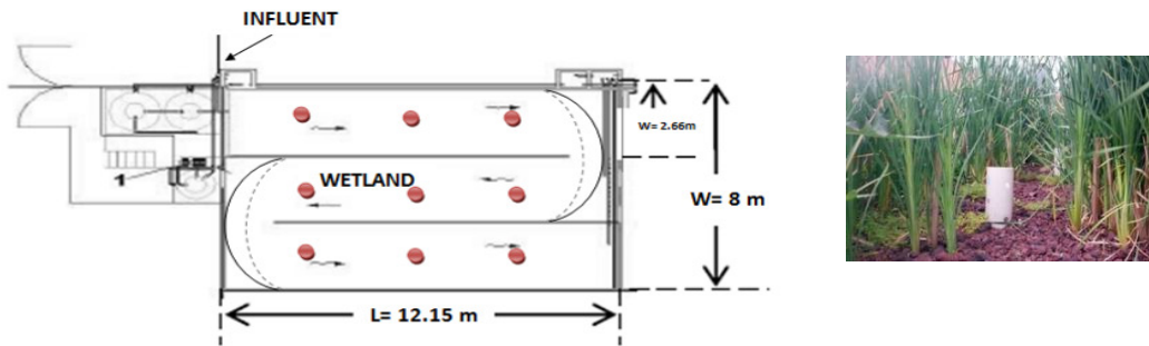
Fig. 3: (3a).Outline of treatment system by subsurface wetland of horizontal flow.
