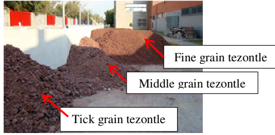
Fig. 4: Selection of three grain sizes for substrate of built wetland.
