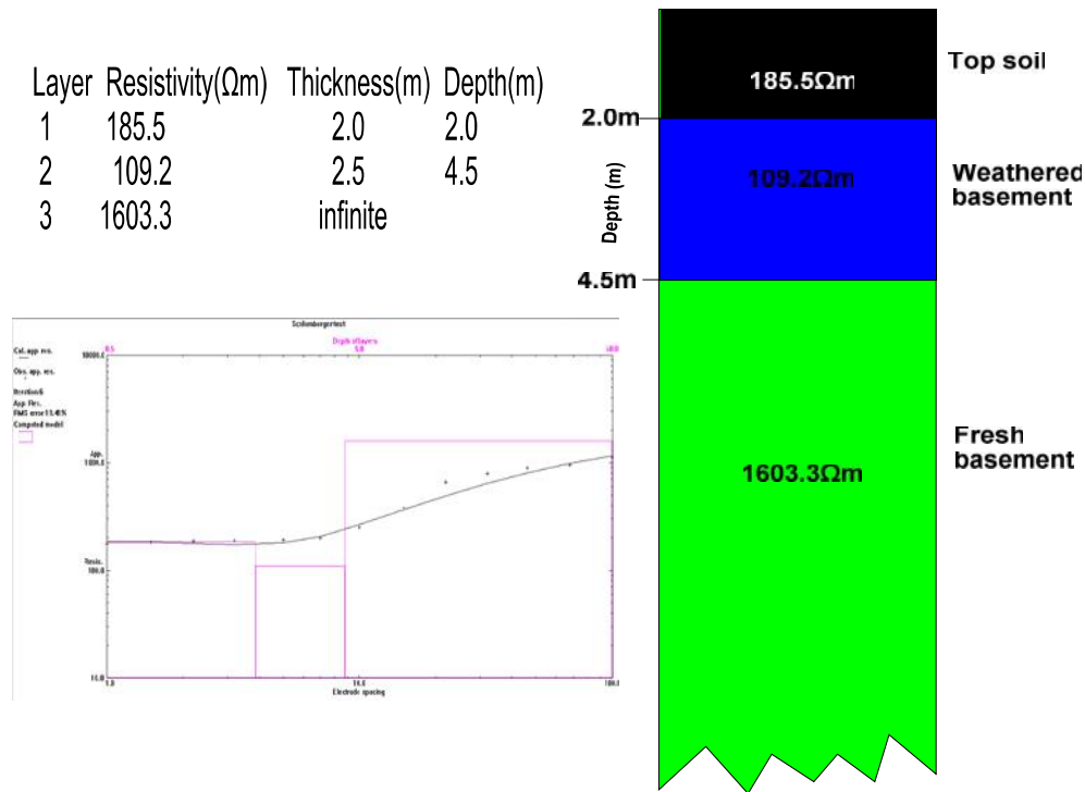
Fig. 5 Sounding Curve and Geoelectric Unit of VES 2 (Staff School, Zaria)
