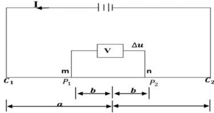
79 80 Fig. 2 General four (4) electrode configuration for resistivity measurement
