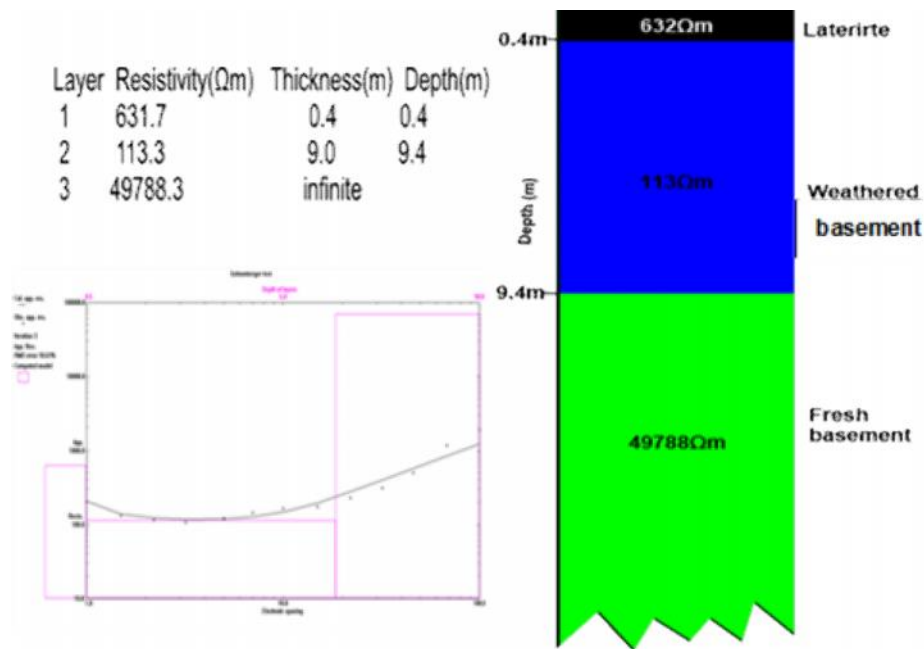
Fig.7 Sounding Curve and Geoelectric Unit of VES 1 (ABU Gymnasium, Zaria)
