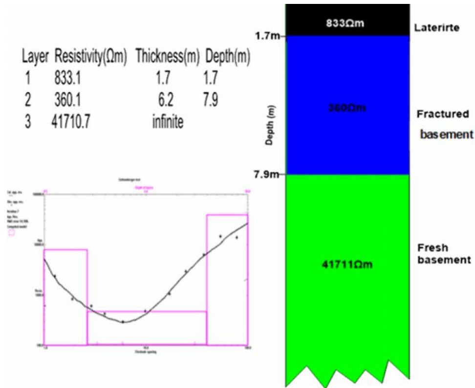
Fig. 6 Sounding Curve and Geoelectric Unit of VES 1 (BZ, Zaria)
