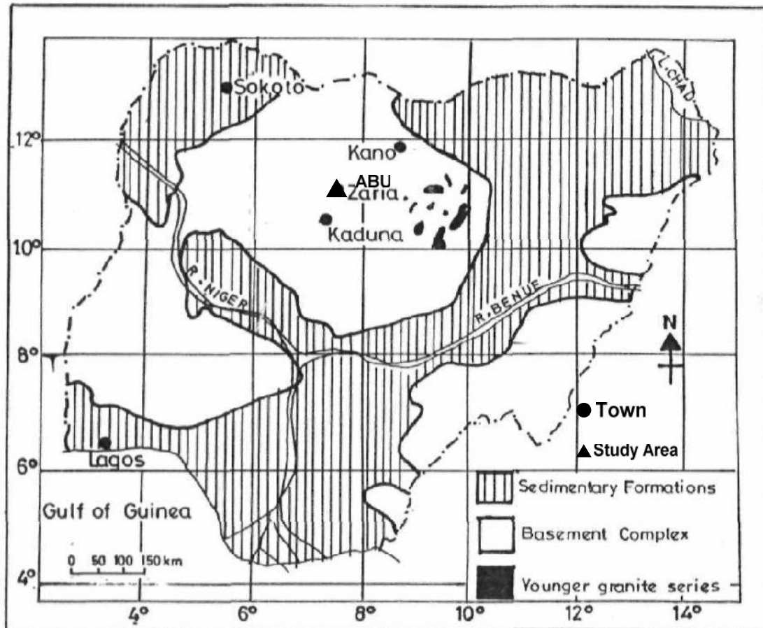
51 Fig. 1a: Geology Map of Nigeria (after Abdullahi et al [9])
