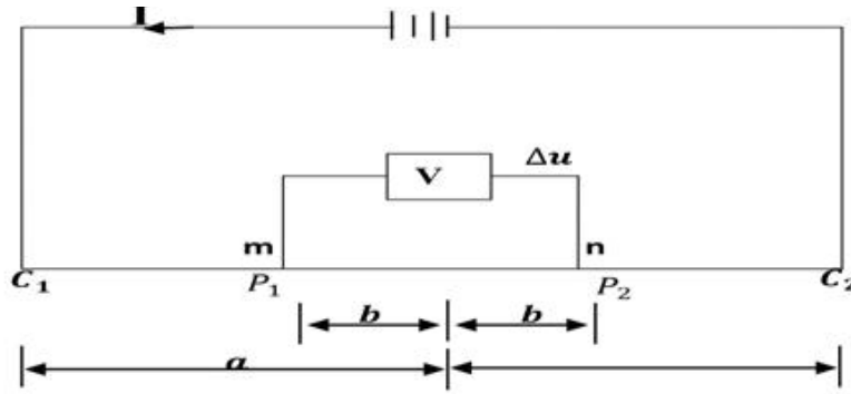
Fig. 3 Generalized Schlumberger electrode configuration resistivity measurement
