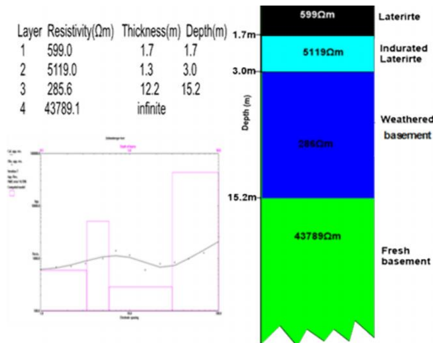
Fig. 4 Sounding Curve and Geoelectric Unit of VES 1 (Waterworks Base, Zaria)
