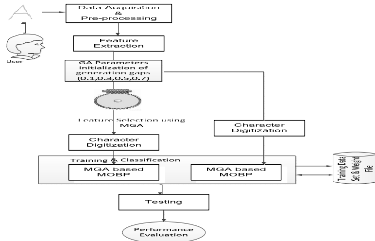
Figure 1: Block diagram of the Developed Online Handwritten Character Recognition Model
