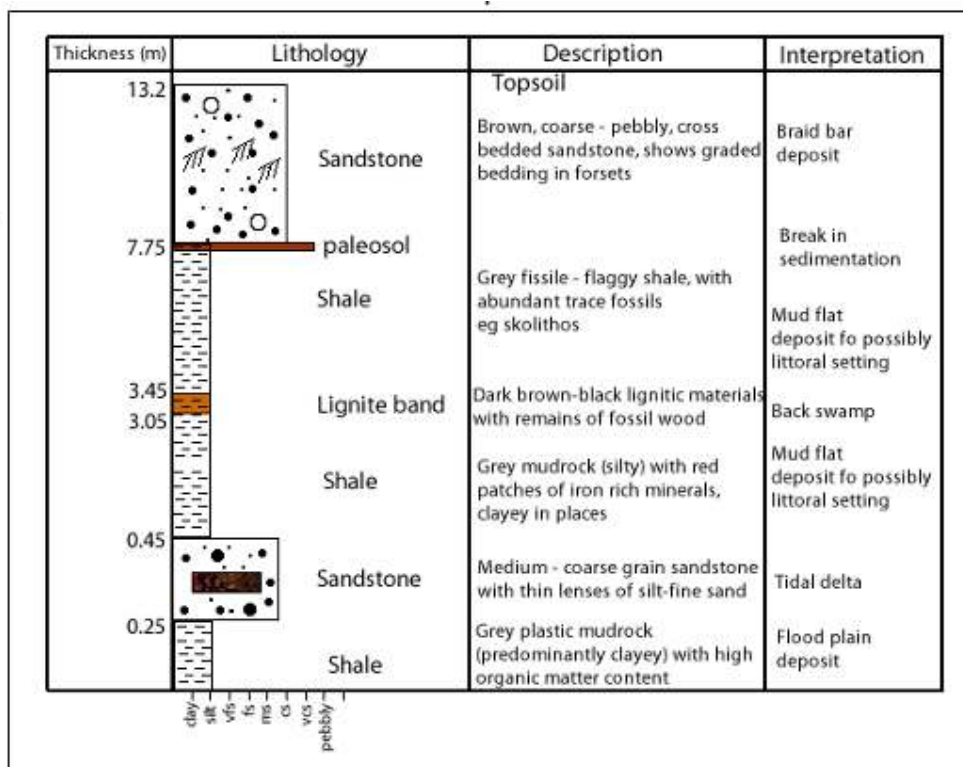
Figure 4: Lithologic section for the road-cut of part of the Benin Formation exposed near Tinapa, Calabar.
