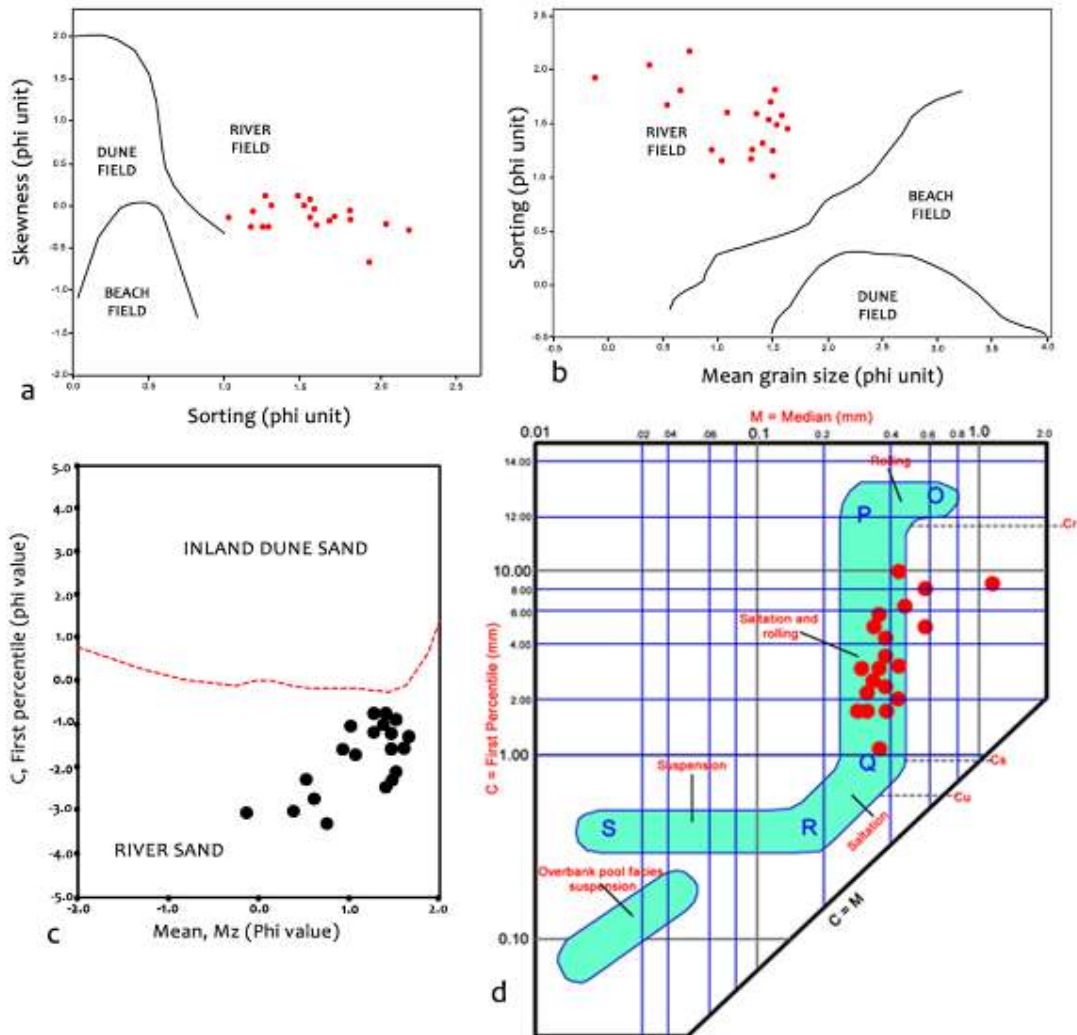
Figure 5: (a) Bivariate plot of skewness against sorting (Martins [13]), (b) Bivariate plot of Sorting against mean grain size (Martins, [13]), (c) Bivariate plot of the first percentile against mean grain size [15] and (d) C-M diagram for characterization of the mode of transportation (Modified from Passega, [16])
