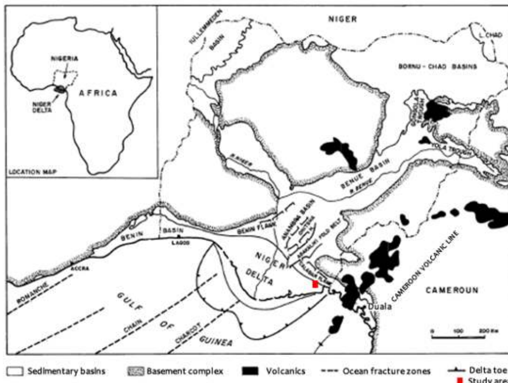
Fig. 2: Regional setting of the Paleogene – Recent Niger Delta (Modified after Knox and Omatsola [6])
