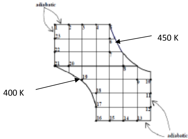
Fig. 7 : Grid Section of a Arbitrary Slab with Mixed Boundaries Arbitrary Slab with Mixed Boundaries
