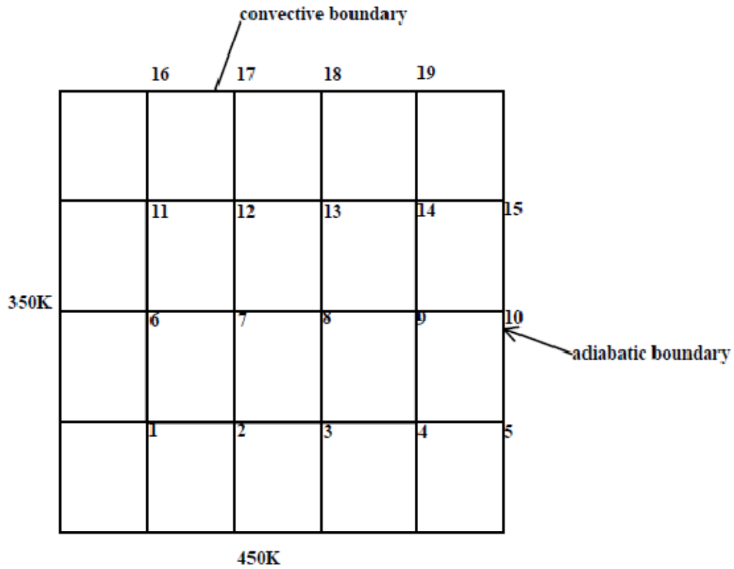
Fig. 4: Rectangular Slab with Mixed Boundaries
