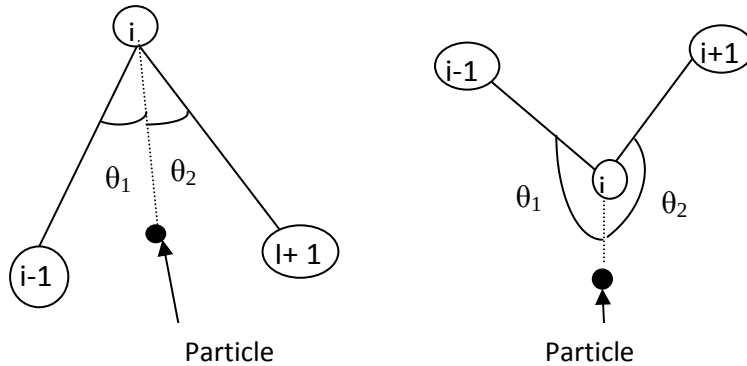
Fig. 2: Possible Particle Positions Close to the Boundary
