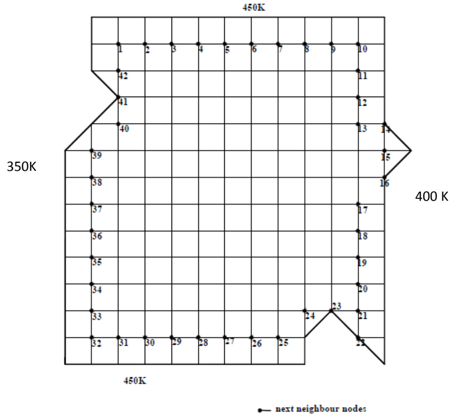
Fig. 5: Arbitrary Shaped Slab with Selected Next Neighbour nodes
