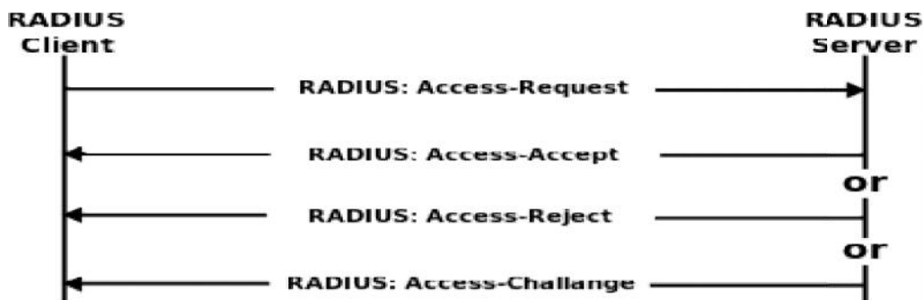
Fig. 2.2: RADIUS Authentication and Authorization Flow (M'Raihi, 2011)
