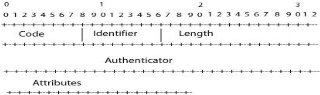
Fig. 2.5: RADIUS Packet Format (Rigney, 2007)
