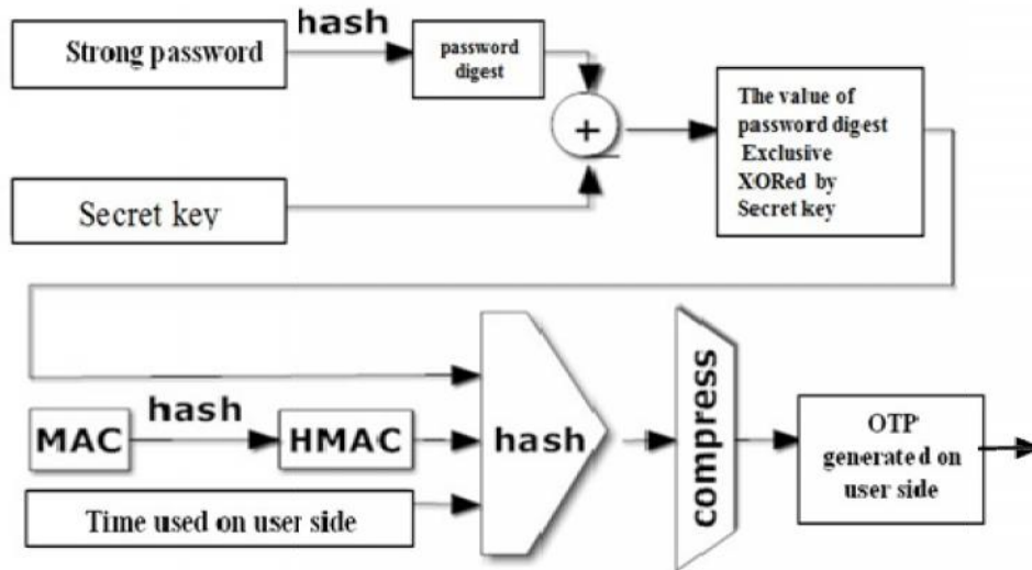
Fig. 2.9: OTP Generation (Xuguang, 2012)
